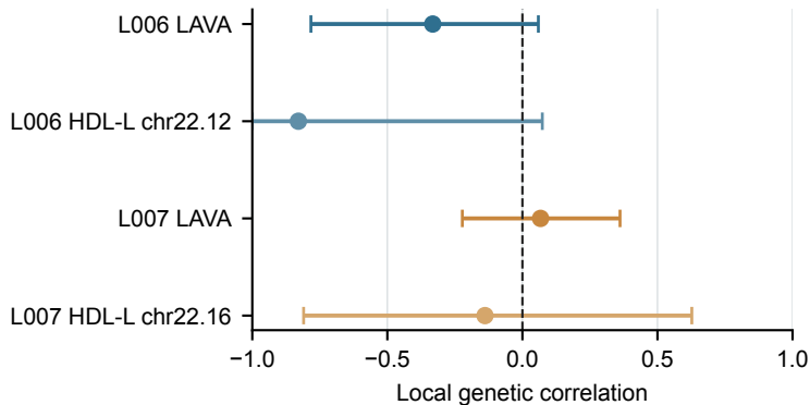
LAVA versus overlapping HDL-L blocks
