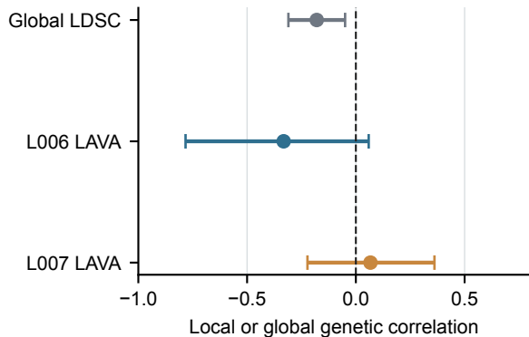
Global signal and two-locus sensitivity
