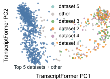
C Study-origin structure
