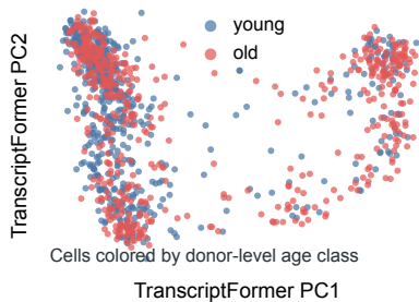
B Donor-level age class
