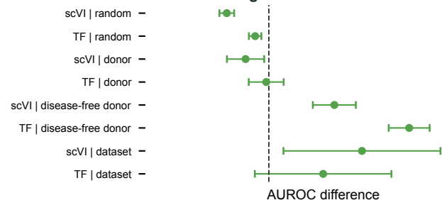
G Embedding AUROC minus metadata-only
