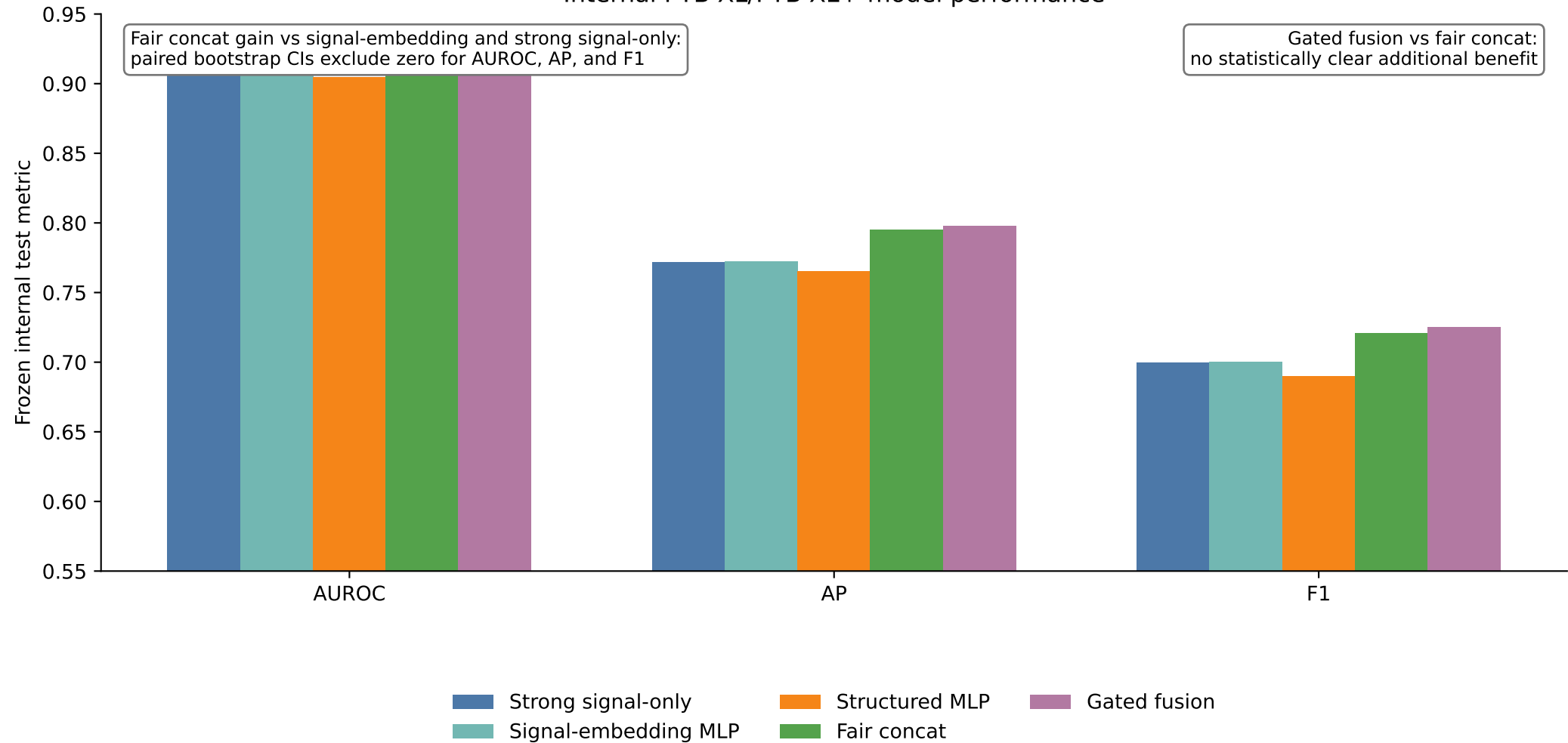
Internal PTB-XL/PTB-XL+ model performance
