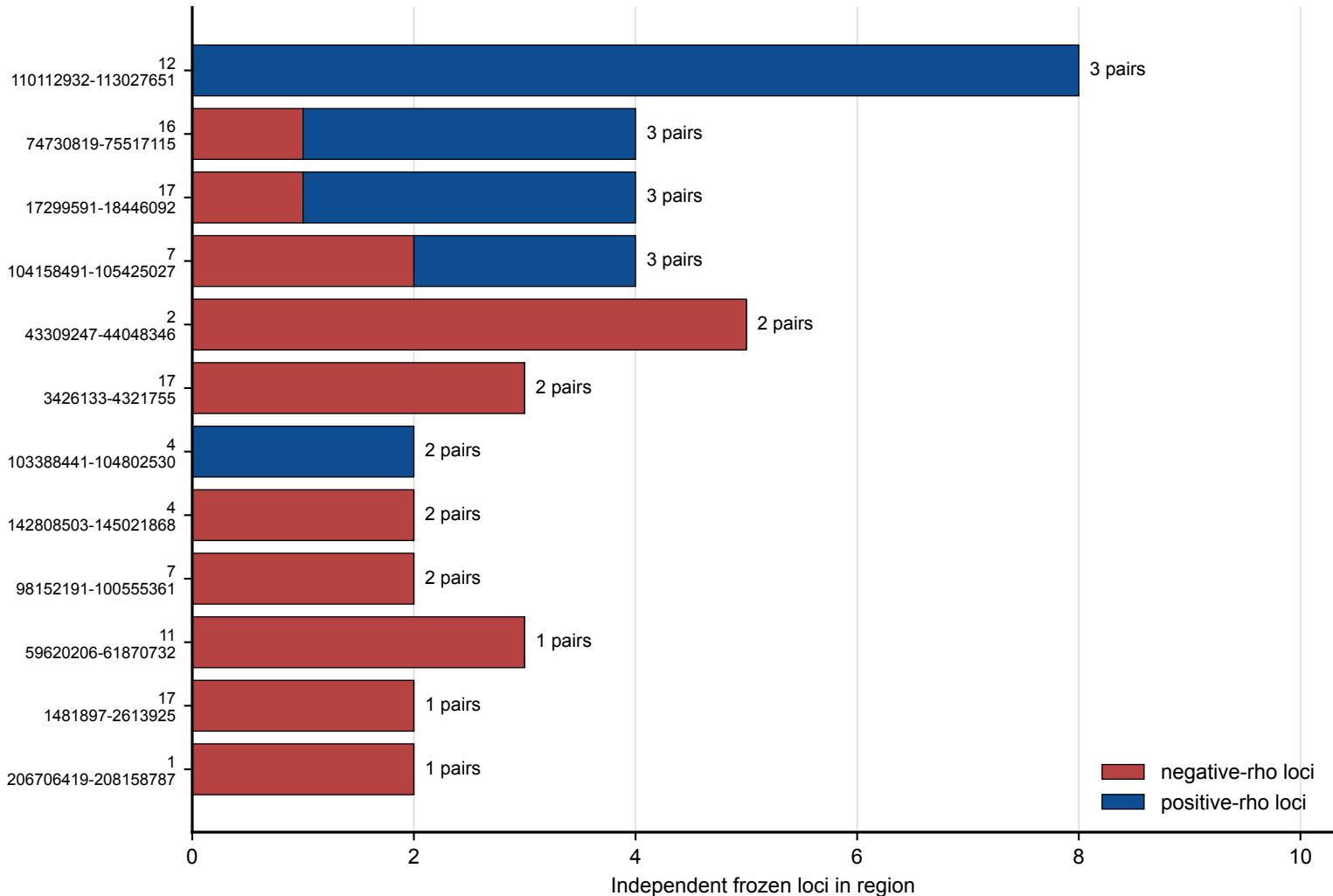
Figure 3C | Recurrent cross-pair regions
