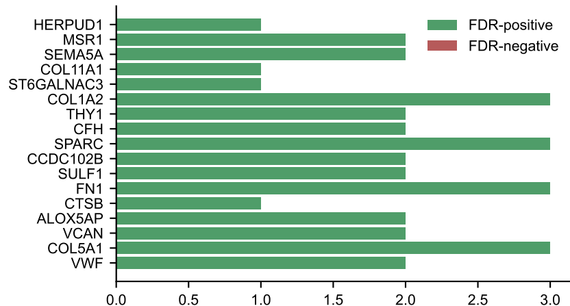
Bulk FDR direction
