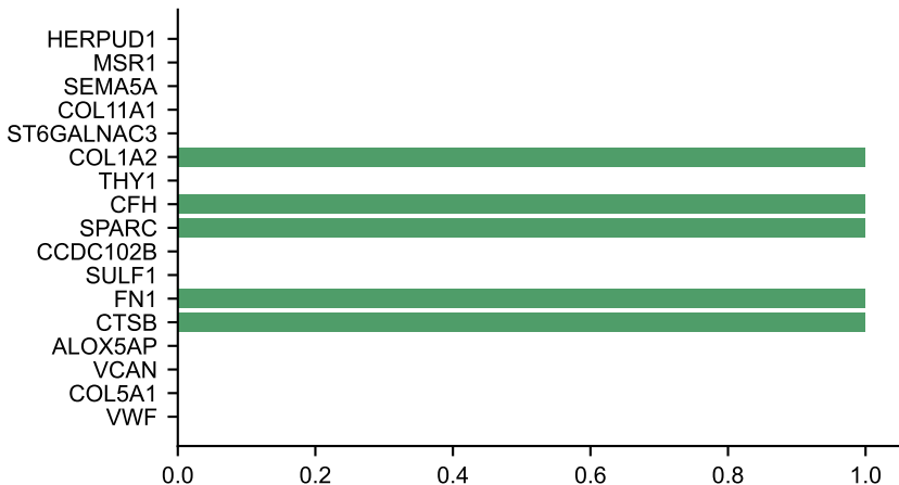
Archived scRNA evaluability
