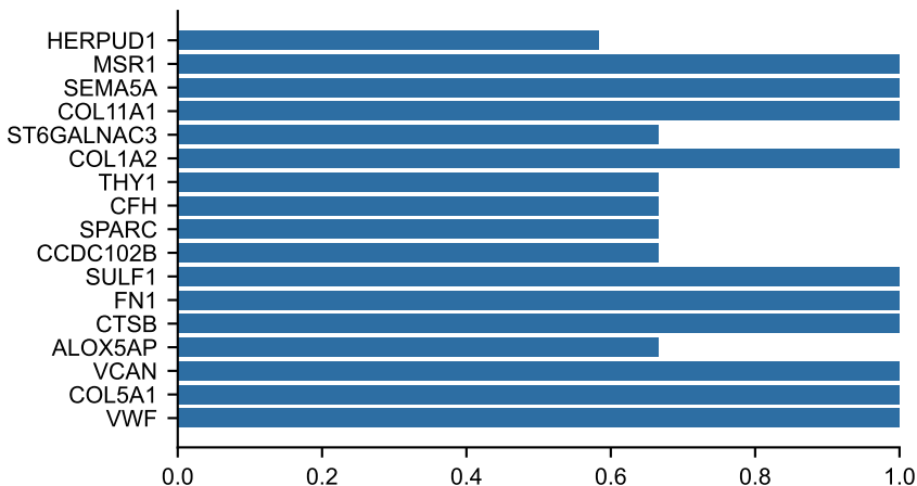
Bulk median LOO concordance
