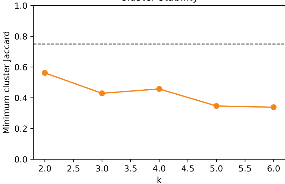
Cluster stability
