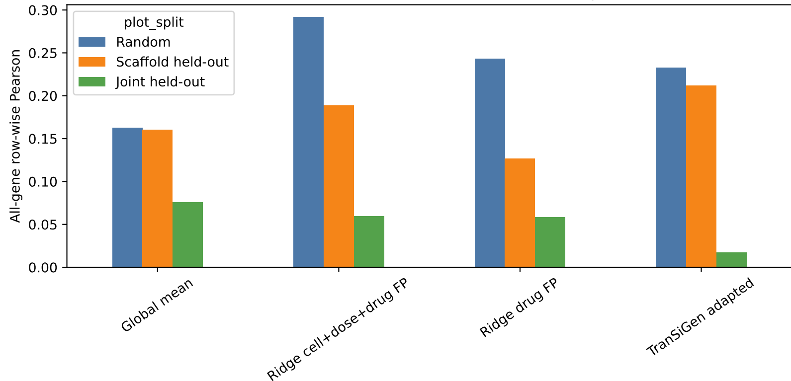
Sci-Plex 3 model stress test with TranSiGen adaptation
