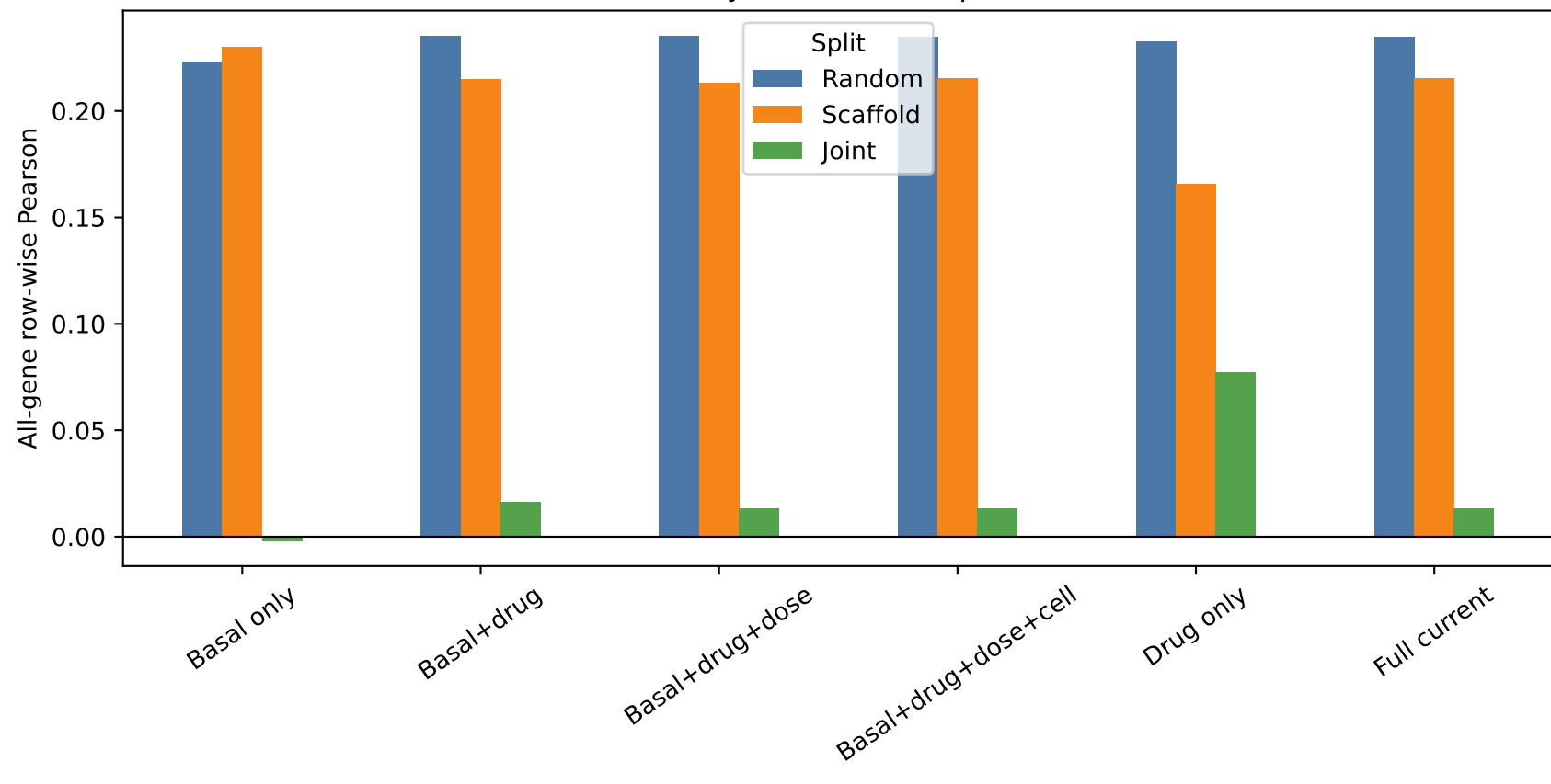
TranSiGen-style Sci-Plex 3 input ablation
