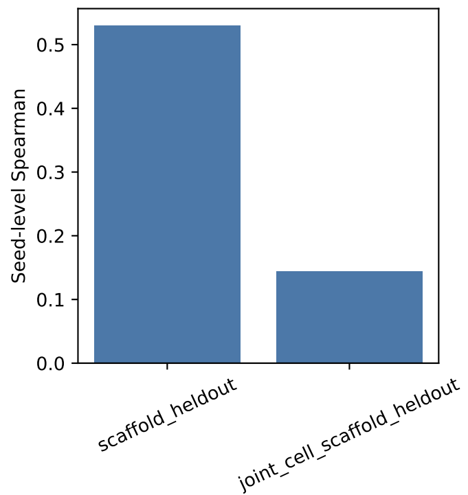
Random-rank transfer
