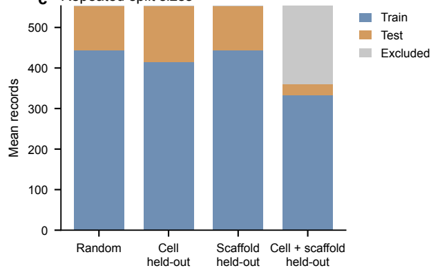
c Repeated split sizes
