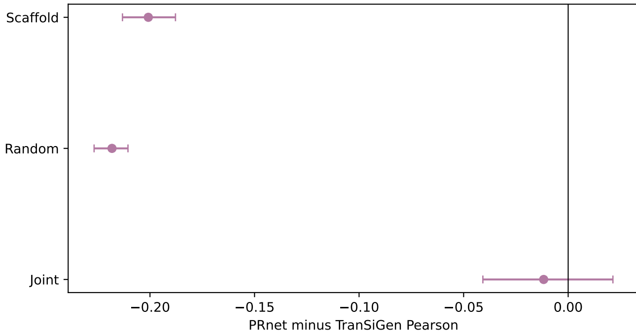
Paired PRnet vs TranSiGen difference
