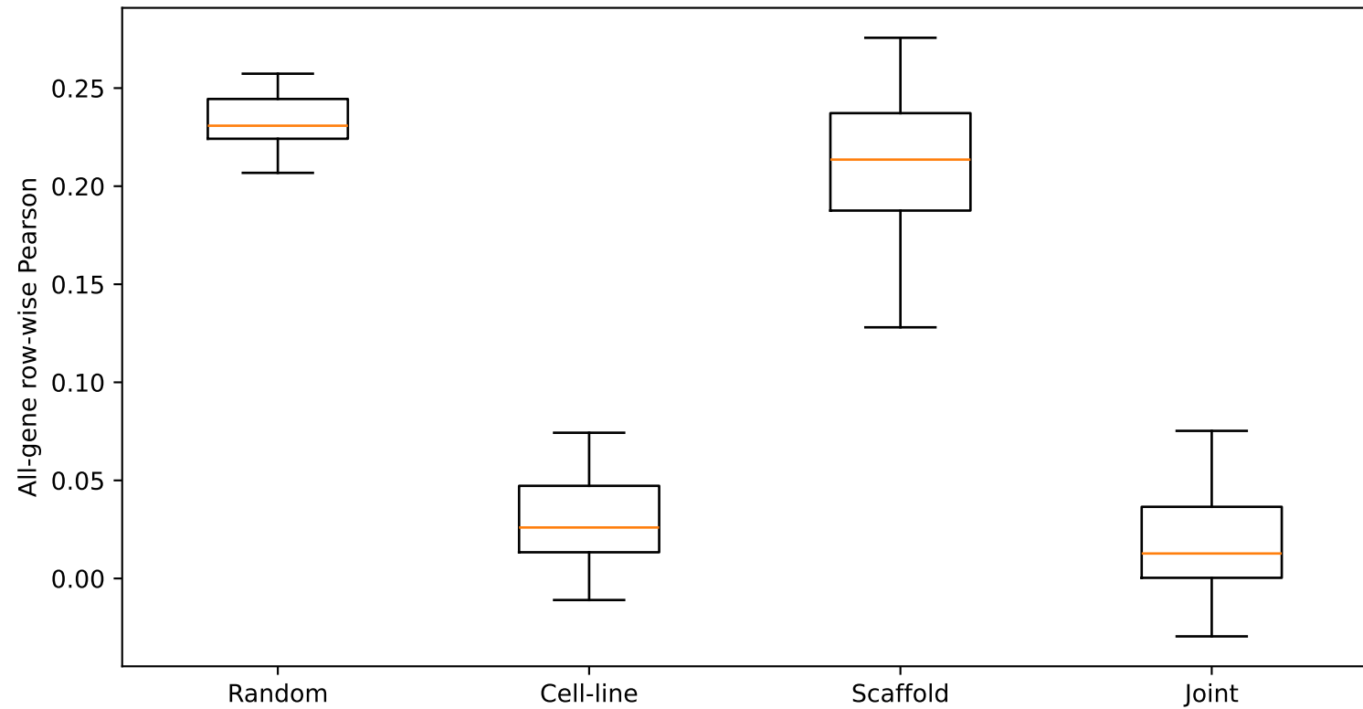
TranSiGen ablation seed-level distributions
