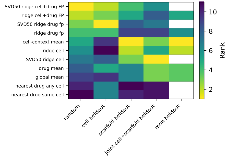
openproblems neurips2023
