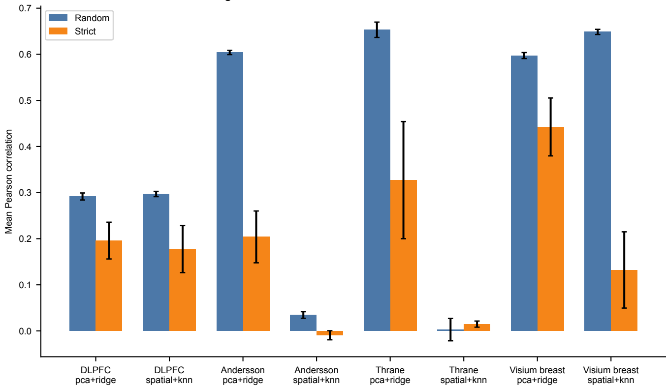
Random and strict evaluation diverge across datasets
