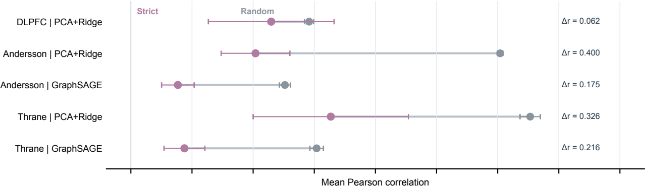
a Subject-held-out evaluation attenuates random-split performance
