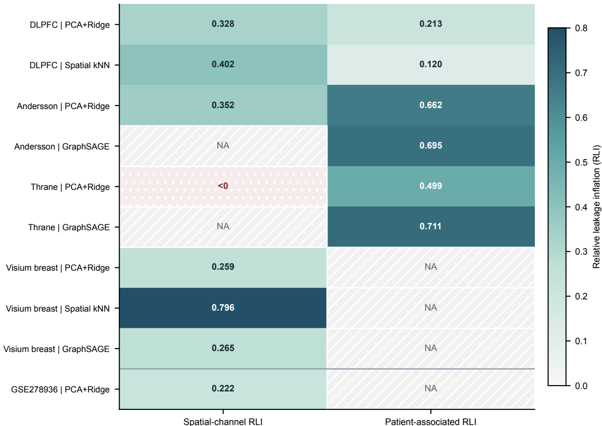
Two-channel landscape of apparent generalization inflation
