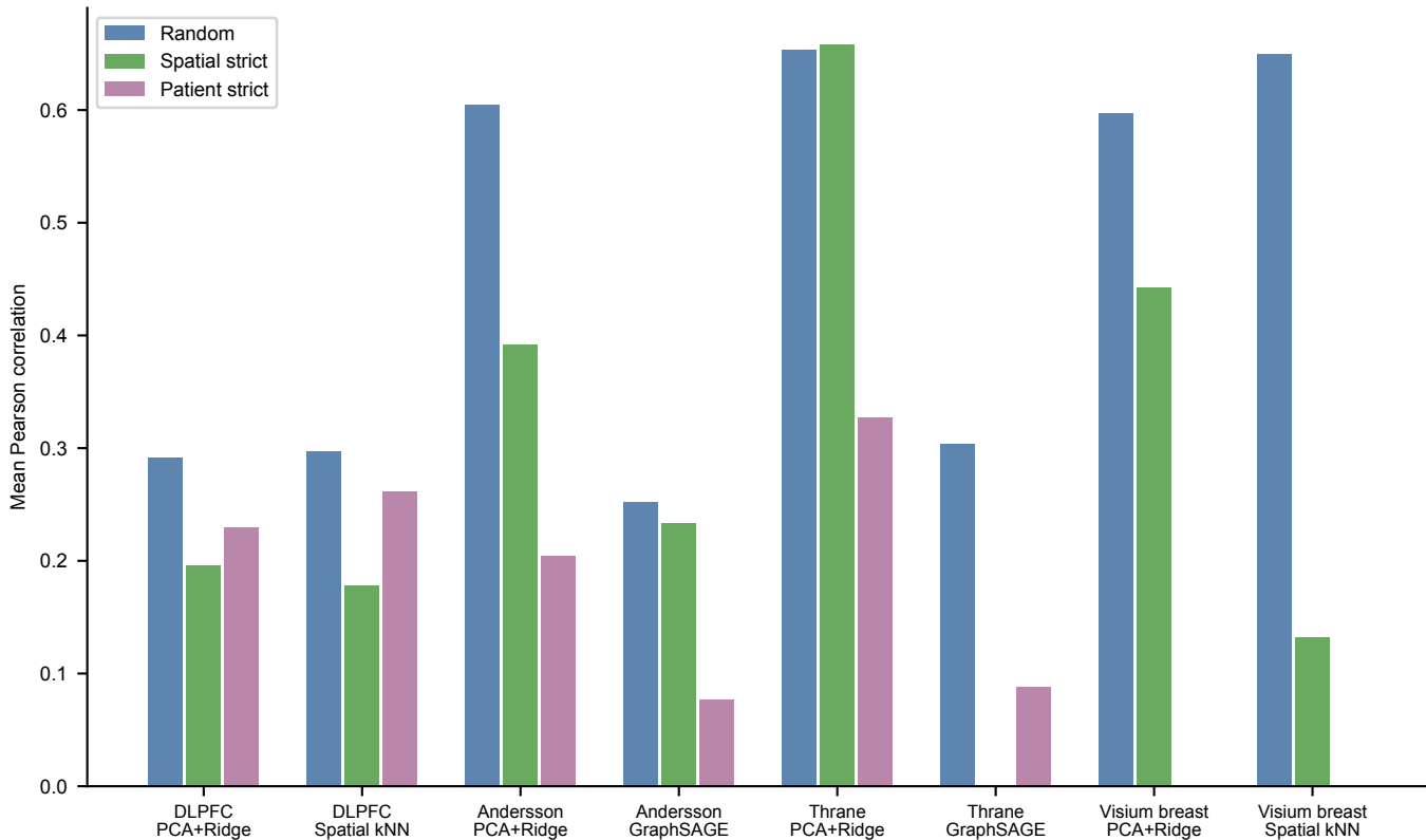
Model behavior changes with evaluation tier
