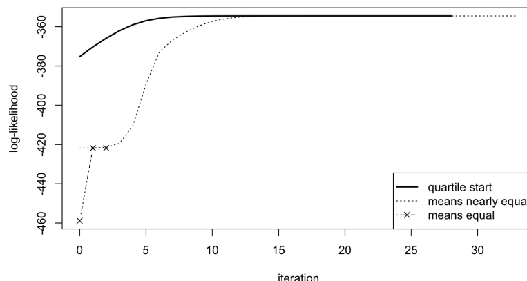
Figure 21.2: Log-likelihood of the given data as a function of the iteration number for the EM algorithm, for the start with quartile-spaced means (solid line), for the start with nearly equal means (dotted line) and for the start with equal means (dash-dotted line with crosses). The trace of the start with interchanged means coincides with the solid line.
