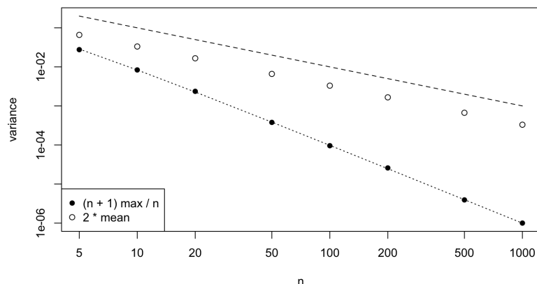
Figure 15.1: Simulated variances for (n+1) \max_i X_i/n (filled circles) and 2\bar{X} (open circles), for the uniform parameter \theta = 1 , on logarithmic axes. The dashed line shows the value \theta^2/n from the Cramer–Rao formula. The dotted line shows the exact variance \theta^2/(n(n+2)) from example 13.6.
