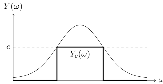
Figure 2.1: The random variable Y and the variable Y_c from the proof of Markov's inequality, as functions of the outcome \omega . Since Y_c is never above Y , its mean c\mathbb{P}(Y \geq c) is at most \mathbb{E}(Y) .
