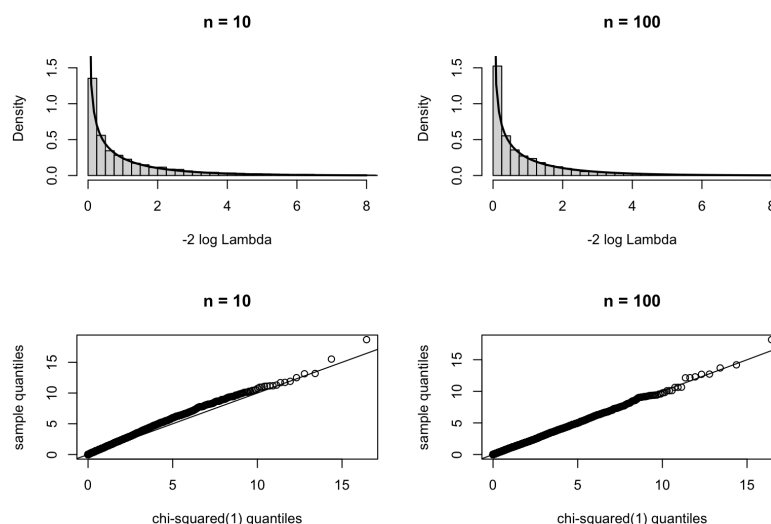
Figure 24.2: The likelihood-ratio statistic W = n \log(1 + t^2/(n - 1)) simulated 10000 times under H_0 for n = 10 (left) and n = 100 (right). Top: histograms with the density of the chi-squared distribution with one degree of freedom (truncated at 8). Bottom: the sorted values of the test statistic against the quantiles of the chi-squared distribution with one degree of freedom, with the identity line.
