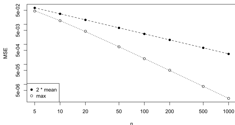
Figure 9.2: Simulated mean squared errors for 2\bar{X} (filled circles) and \max_i X_i (open circles), for the uniform parameter \theta = 1 , on logarithmic axes. The exact values \theta^2/(3n) (dashed line) and 2\theta^2/((n+1)(n+2)) (dotted line) are also shown.
