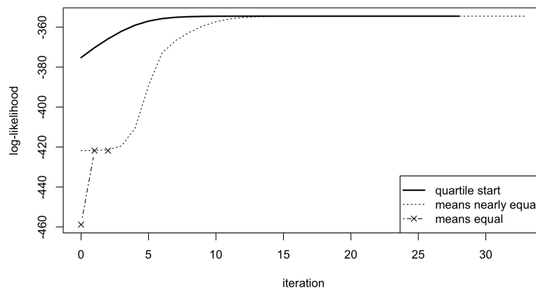
Figure 21.2: Log-likelihood of the given data as a function of the iteration number for the EM algorithm, for the start with quartile-spaced means (solid line), for the start with nearly equal means (dotted line) and for the start with equal means (dash-dotted line with crosses). The trace of the start with interchanged means coincides with the solid line.
