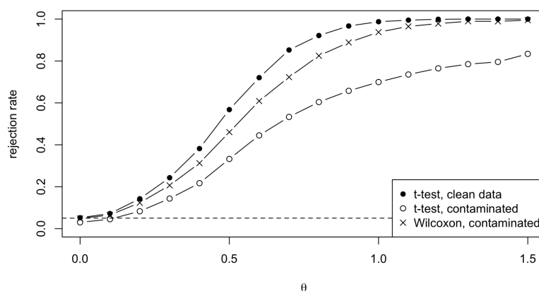
Figure 30.2: Estimated power functions at level 0.05 for 2000 samples of size n = 20 , for the t -test on clean, normally distributed data (filled circles), the t -test on contaminated data (open circles), and the Wilcoxon signed-rank test on contaminated data (crosses).
