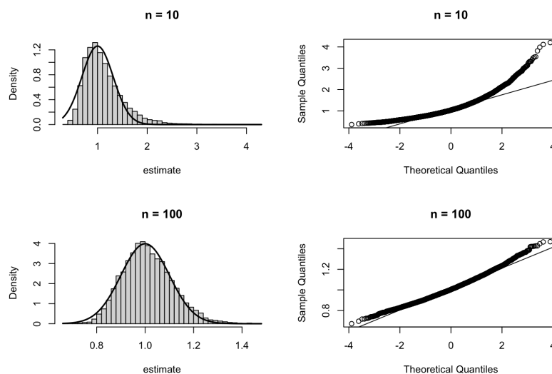
Figure 12.1: The sampling distribution of \hat{\theta} = 1/\bar{X} for the exponential model with \theta = 1 : histograms with the normal approximation overlaid (left column) and normal quantile plots (right column), for 10000 samples of size n = 10 (top row) and n = 100 (bottom row).
