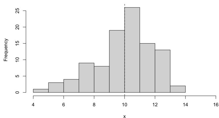
Figure 3.1: A simulated sample of n = 100 observations from a normal distribution with mean \mu = 10 and variance \sigma^2 = 4 . The dashed line gives the sample mean.
