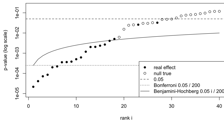
Figure 30.1: The 40 smallest of 200 p -values against their rank on a logarithmic scale: real effects (filled circles) and true null hypotheses (open circles), with the raw level 0.05 (dashed), the Bonferroni level 0.05/200 (dotted) and the Benjamini–Hochberg line 0.05 i/200 (solid).
