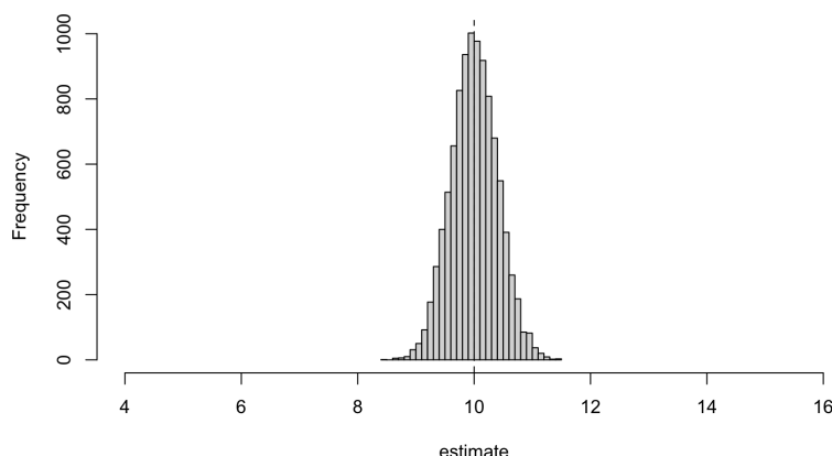
Figure 3.2: The sampling distribution of the sample mean \bar{X} for n = 25 : a histogram of 10000 simulated estimates, where the true mean \mu = 10 is marked by the dashed line. The axis is the same as in figure 3.1.
