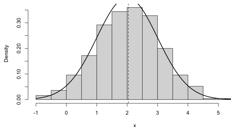
Figure B.1: A histogram on the density scale, with the true density overlaid and the sample mean marked by a dashed line.
