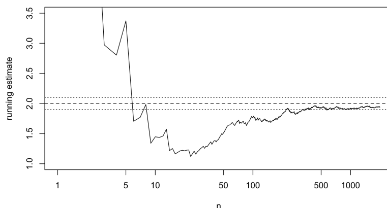
Figure 9.1: The running estimate 1/\bar{X}_n for the exponential rate \theta = 2 , plotted against n on a logarithmic axis. The truth is given by the dashed line, the band \theta \pm 0.1 is given by the dotted lines.
