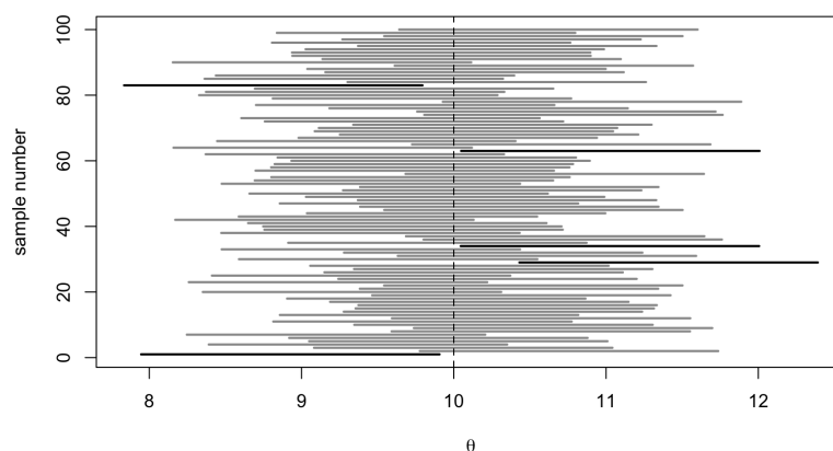
Figure 27.1: One hundred 95% confidence intervals for the mean of a N(\theta, 4) sample of size n = 16 , with true value \theta = 10 (dashed line). The grey intervals cover the truth, the black intervals do not.
