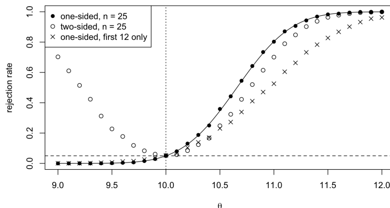
Figure 24.1: Estimated power functions for three level 0.05 tests for H_0: \theta = 10 , using 5000 samples of size n = 25 for each grid point: one-sided z -test (filled circles), two-sided z -test (open circles) and one-sided z -test on the first 12 observations only (crosses). For comparison, the line gives the exact power function of the one-sided test from lecture 20.
