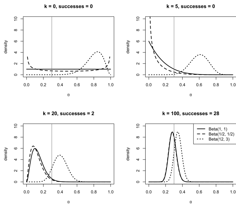
Figure 27.2: Posterior densities for the probability of success in a Bernoulli trial after k = 0, 5, 20 and 100 observations of one simulated sequence with \theta = 0.3 (grey vertical line), for the priors Beta(1, 1) (solid), Beta(1/2, 1/2) (dashed) and Beta(12, 3) (dotted).
