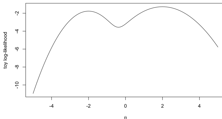
Figure 18.1: The toy function with the two peaks. The peak found by optim depends on the starting point. If optimise is used, it returns the lower peak, despite the interval containing both peaks.
