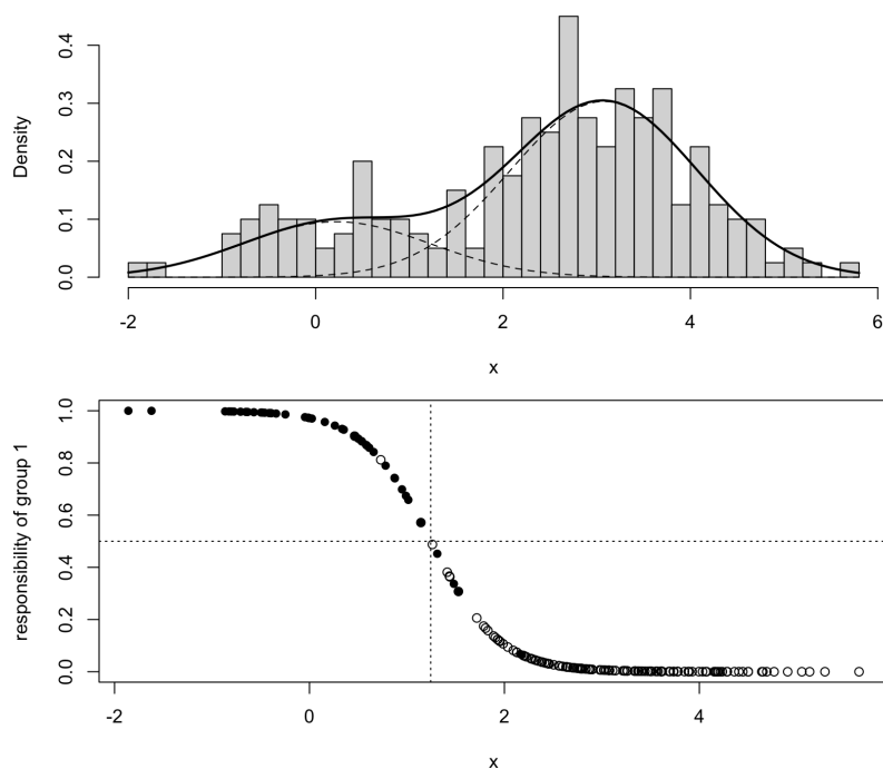
Figure 21.1: The fitted mixture density with its two weighted components (top panel) and the responsibilities of group 1 at the fixed point as a function of the observations (bottom panel). The filled circles give the observations which were assigned to group 1. The dotted lines give the responsibility 1/2 and the crossing point 1.244.
