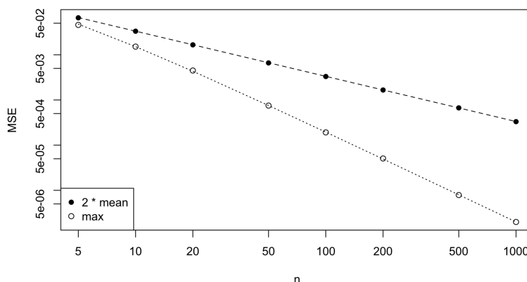
Figure 9.2: Simulated mean squared errors for 2\bar{X} (filled circles) and \max_i X_i (open circles), for the uniform parameter \theta = 1 , on logarithmic axes. The exact values \theta^2/(3n) (dashed line) and 2\theta^2/((n+1)(n+2)) (dotted line) are also shown.
