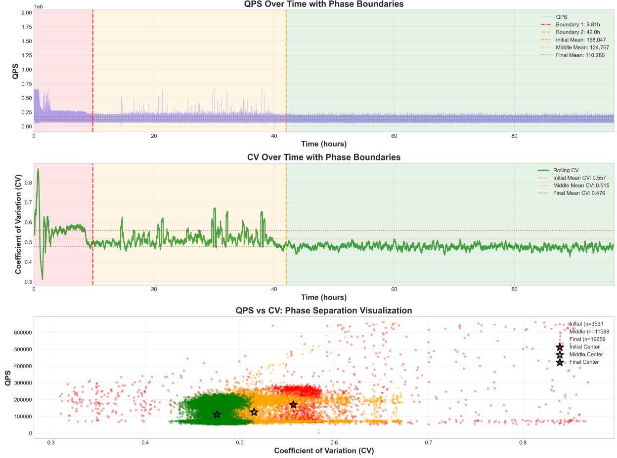
Figure 2: Three-Phase Segmentation Justification: This comprehensive visualization demonstrates the empirical justification for dividing RocksDB performance into three distinct operational phases based on QPS and CV metrics. The upper panel shows QPS evolution over time with phase boundaries at 9.81h and 42.0h, along with phase-specific mean QPS levels (Initial: 168,047; Middle: 124,767; Final: 110,280 ops/sec), clearly illustrating the 25.8% QPS reduction from Initial to Middle and 11.6% reduction from Middle to Final. The middle panel shows CV evolution, revealing consistent decreasing volatility across phases (Initial: 0.557; Middle: 0.515; Final: 0.476) with approximately 7.5-7.6% reduction at each boundary. The lower panel is a QPS-CV scatter plot with phase-specific coloring, demonstrating clear separation between phases: Initial phase data (red) shows high QPS and high CV cluster, Middle phase (orange) shows intermediate values, and Final phase (green) shows lower QPS but lowest CV, indicating mature steady-state. The distinct clusters in the scatter plot, combined with the phase-specific mean centers marked by stars, validate that three-phase segmentation captures meaningful operational differences rather than arbitrary divisions.
