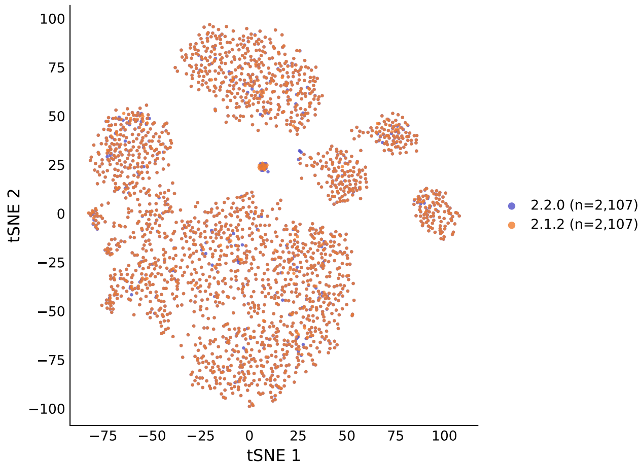
Merge of 2.2.0 and 2.1.2 on shared embedding (tSNE), n=4,214
