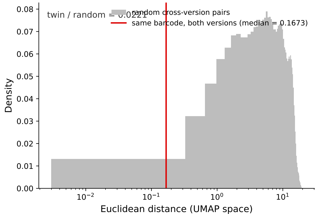
UMAP space: twin-copy distance vs random pairing
