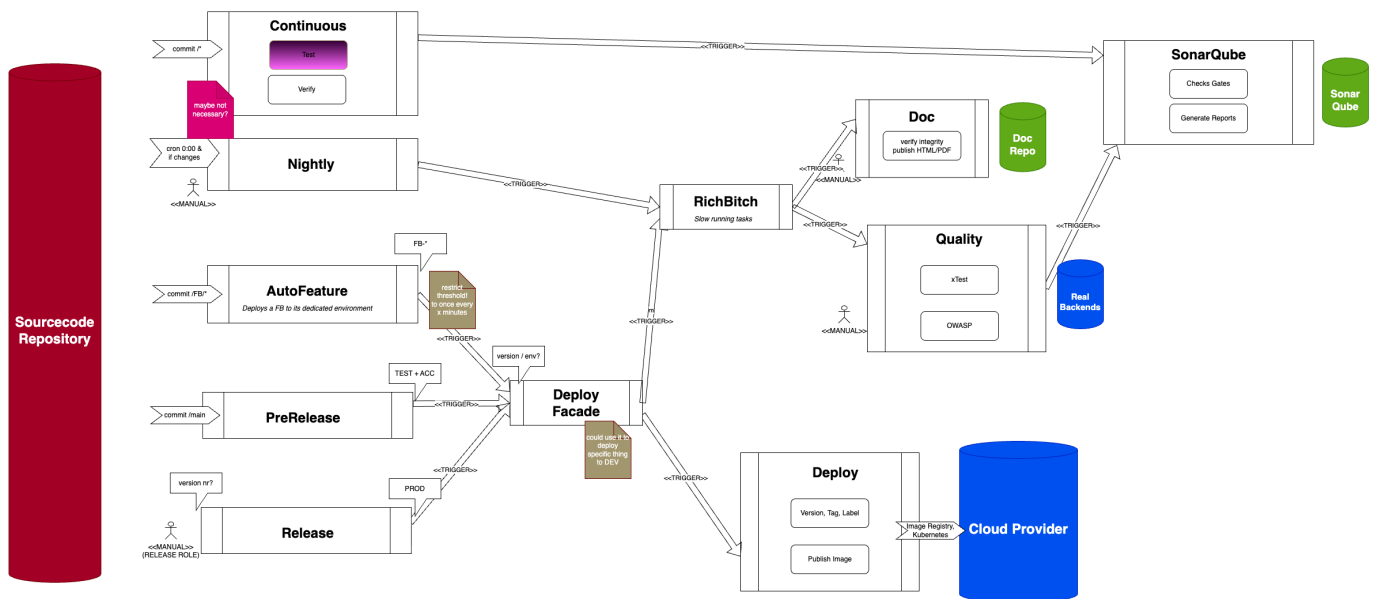
Figure 5. Sketching a build pipeline overview
