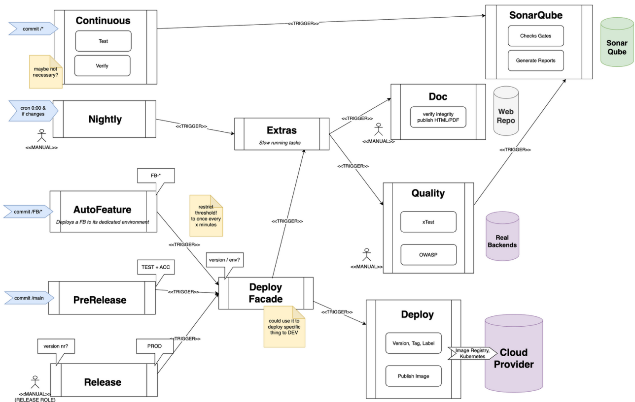
Figure 6. Sketching a build pipeline overview
