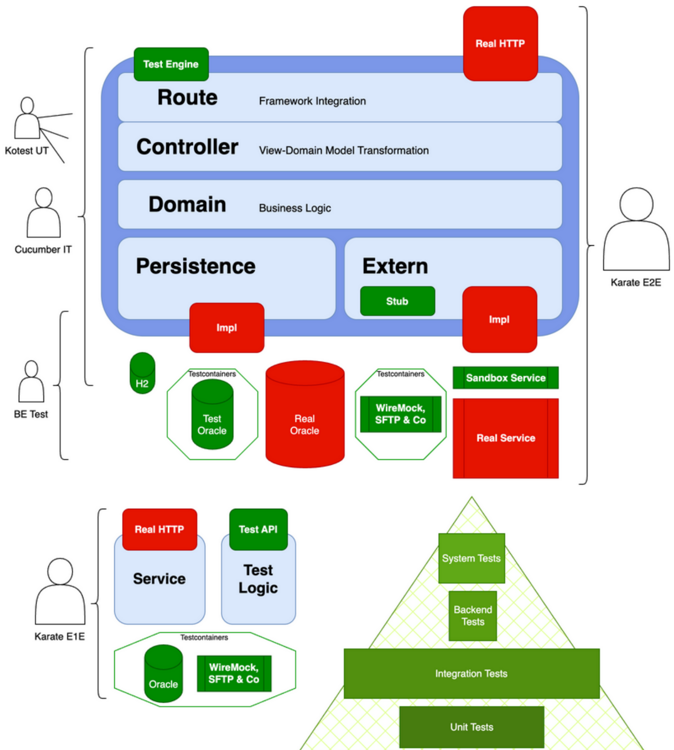
Figure 5. Simplified view from different test strategies onto the application boundaries
