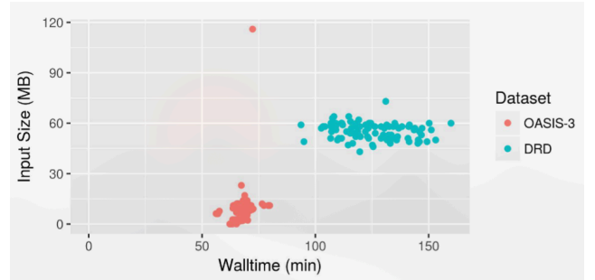
Fig. 6. 2020 study result for SLANT CPU Singularity walltime on two separate datasets
