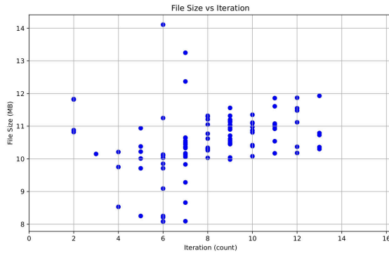
Fig. 14. Atropos number of iterations vs file size
