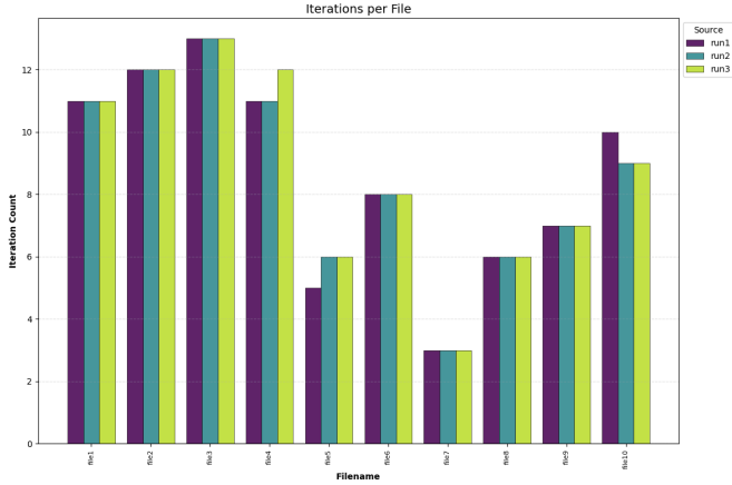
Fig. 13. Atropos number of iterations across 3 different runs
