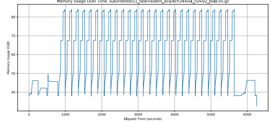
Fig. 5. SLANT CPU Singularity memory profile for all 128 threads
