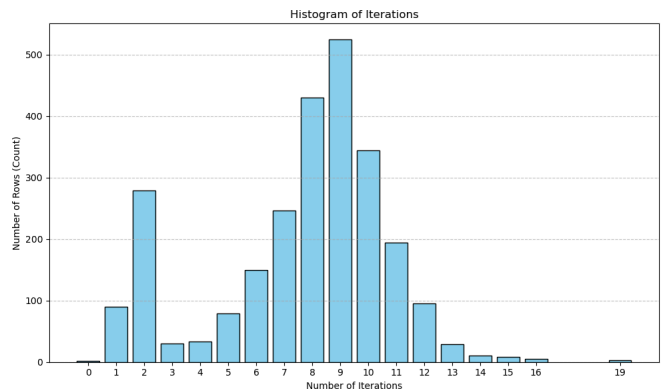
Fig. 12. Atropos histogram of number of iterations to convergence
