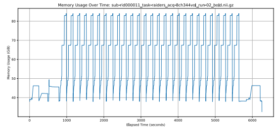
Fig. 4. SLANT CPU Singularity memory profile for all 128 threads
