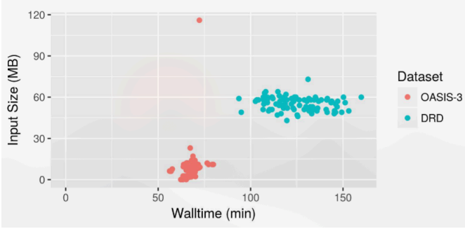
Fig. 5. 2020 study result for SLANT CPU Singularity walltime on two separate datasets
