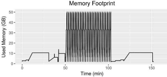
Fig. 6. 2020 study result for SLANT CPU Singularity memory profile on an DRD data
