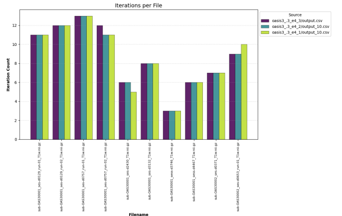
Fig. 13. Atropos number of iterations across 3 different runs
