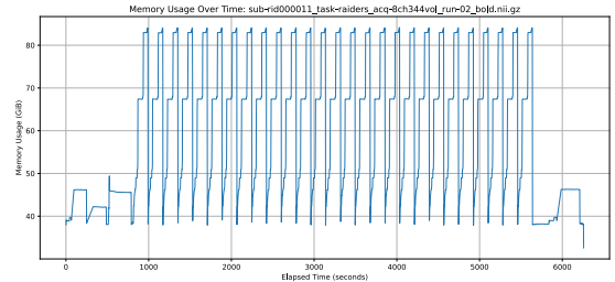
Fig. 4. SLANT CPU Singularity memory profile for all 128 threads
