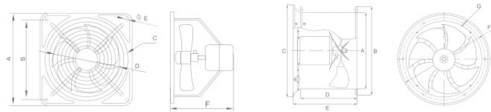
Outline dimensions
