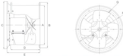
Outline dimensions
