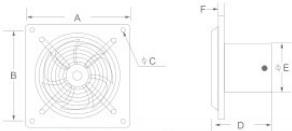
Outline dimensions
