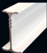
KF2502 (0.132kg/m)
