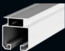
KF1705 (0.154kg/m)
