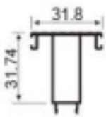
JNW-XT1468 bottom double side frame cover Weight: 0.38kg/m
