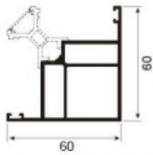
JNW-XT1009 outside 90° slim corner Weight : 1.14 kg/m
