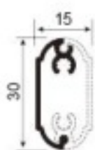
JNW-XT051F two-color grid strip Weight: 0.20kg/m
