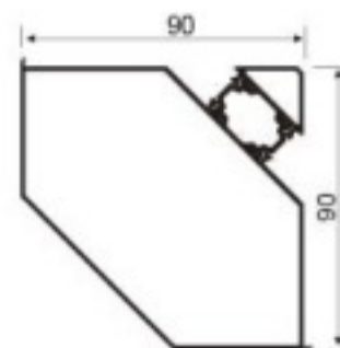
XTC-ZJ90A 90 corner -90° Weight: 1.728kg/m
