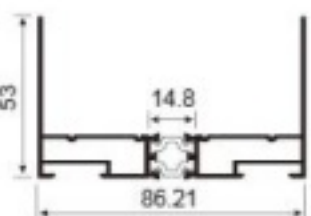
JNW-CT1416F four-rail side seal Weight: 1.34kg/m
