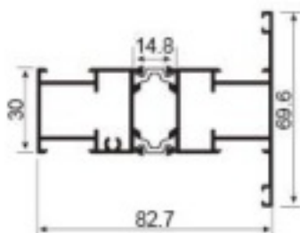
JNW-CT1343G two rail inner frame Weight: 1.54kg/m
