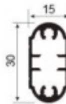
GD-036A integrated grid strip Weight: 0.37kg/m
