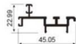
JNW-XT1345 four-rail additional bottom rail Weight: 0.46kg/m
