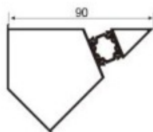
XTC-ZJ90B 90 corner -135° Weight: 1.251kg/m
