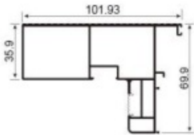
JNW-XT1470 handrail Weight: 1.51kg/m
