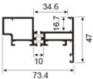
DZ-CT795F slim glass sash Weight : 1.36 kg/m
