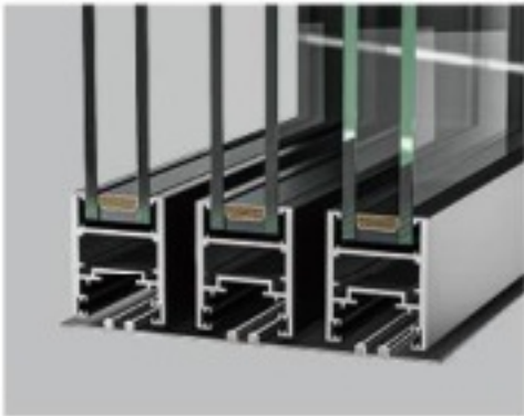
triple-rails flat rail double-row wheel
