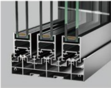
triple-rail higher rail double-row wheel
