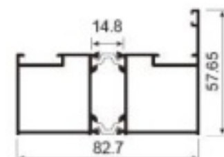
JNW-CT1420F four-rail side seal conversion Weight: 1.40kg/m
