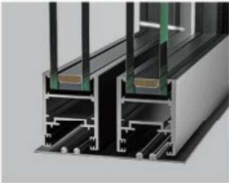
double rails flat rail double-row wheel
