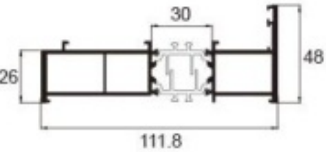
JNW-BK781F 3.0 Outer Frame Weight : 2.15 kg/m
