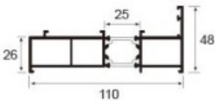
JNW-BK812A injection molded frame Weight : 1.69 kg/m
