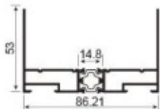
JNW-CT1416F two rail side seal Weight: 1.34kg/m
