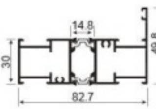
JNW-CT1343E two tracks fixed up and down Weight: 1.49kg/m
