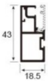
DZ-793 slim screen sash Weight : 0.59 kg/m
