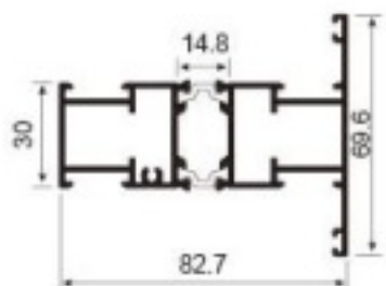
JNW-CT1343G four-rail center column Weight: 1.54kg/m
