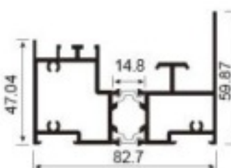
JNW-CT1346S four-rail bottom rail (land) Weight: 1.69kg/m
