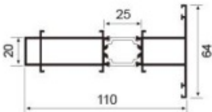
JNW-ZH813A injection molded center post Weight : 1.82 kg/m
