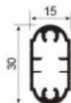
GD-036A integrated grid strip Weight: 0.37kg/m
