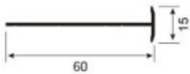
JNW-XT208 frame splicing strip Weight : 0.28 kg/m
