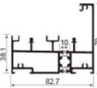
JNW-CT1676F two-track suspended bottom rail(landing) Weight: 2.19g/m
