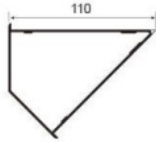
ZJ110B 110 degree corner-135° Weight : 1.13 kg/m
