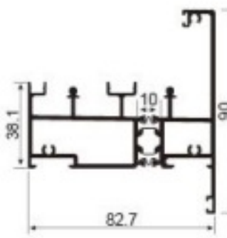
JNW-CT1459F two-track suspended bottom rail Weight: 2.29kg/m
