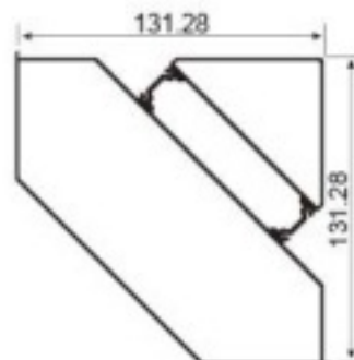
XTC-ZJ130A 130 corner -90° Weight: 2.80kg/m
