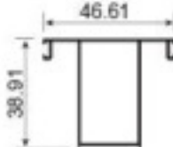
JNW-XT1331 side frame double cover Weight: 0.46kg/m
