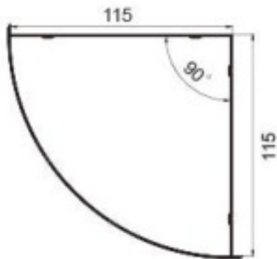
ZJ115A 115 turns -90 degrees Weight : 1.48 kg/m
