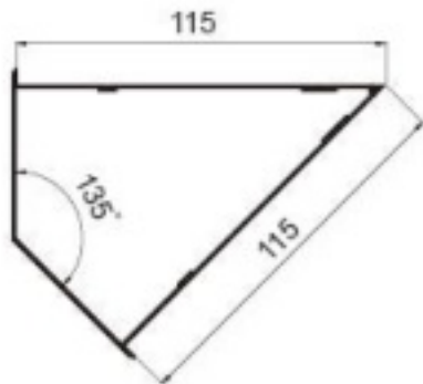
ZJ115B 115 corner-135 degrees Weight : 1.14 kg/m
