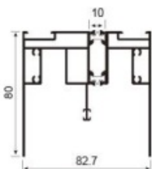
JNW-CT1487F four-rail top rail Weight: 2.32kg/m
