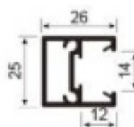
JNW-XT1003 glass guardrail Weight: 0.5kg/m
