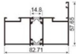
JNW-CT1420F two-track side frame transform Weight: 1.40kg/m
