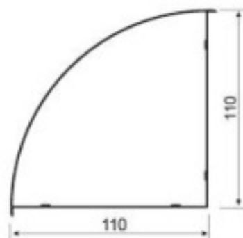
ZJ110A 110 corner -90° Weight: 1.35kg/m
