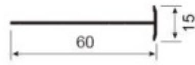
JNW-XT208 frame splicing strip Weight : 0.28 kg/m
