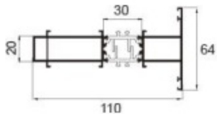
JNW-ZH813F Glue injection center column Weight : 1.92 kg/m
