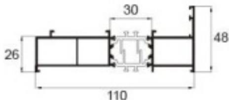
JNW-BK812F Glue injection frame Weight : 1.79 kg/m
