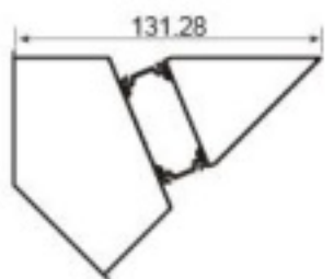
XTC-ZJ130B 130 corner -90° Weight: 1.95kg/m
