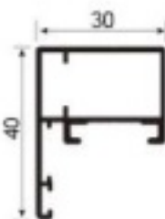
JNW-XT389 clothes drying guardrail frame Weight: 0.50kg/m
