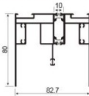
JNW-CT1487F two-track suspended upper rail Weight: 2.32kg/m
