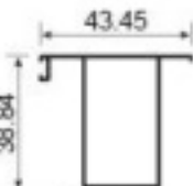
JNW-XT1332F side frame single cover Weight: 0.41kg/m
