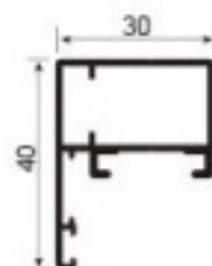
JNW-XT389 clothes drying guardrail frame Weight: 0.50kg/m
