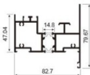
JNW-CT1346F four-rail bottom rail Weight: 1.80kg/m
