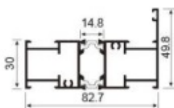
JNW-CT1343E four-rail fixed up and down Weight: 1.49kg/m
