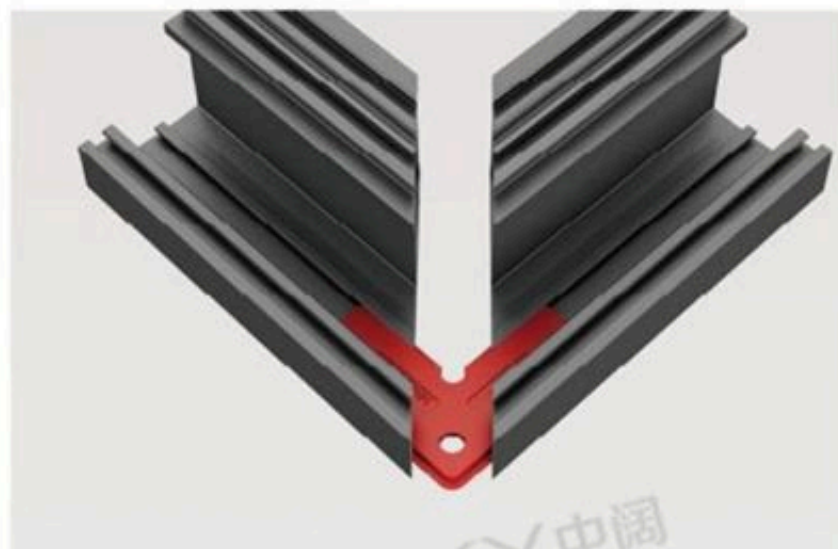
名称: 尼龙组角片 Name: Nylon Corner Connector 材质: PA、PP Material: PA、PP 现货 \ 定制: 非标定制可试配 Non-standard customization can be tried on
