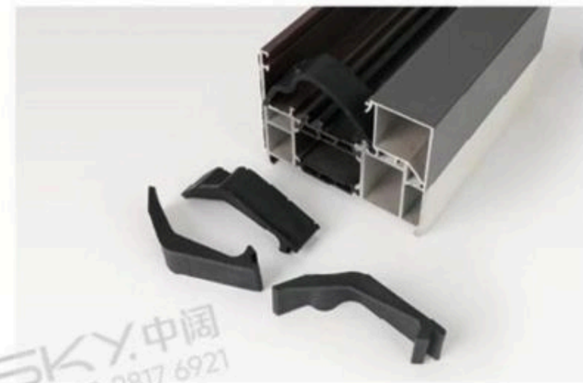
名称: 压线撑子 Name: Crowbar support 材质: PP Material: PP 现货\定制: 非标定制可试配 Non-standard customization can be tried on
