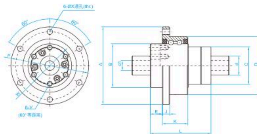
RSF Nut Rotary Ball Spline Specifications and Dimensions Table
