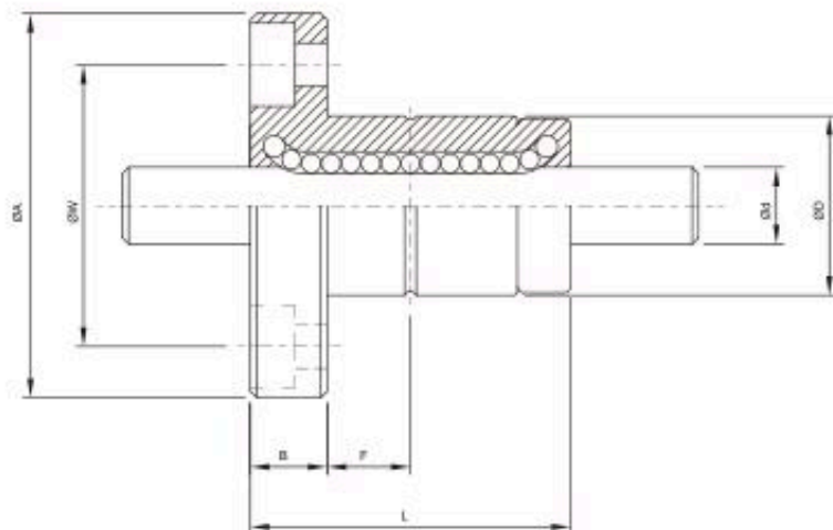
FSLF Series Specification and Size Table
