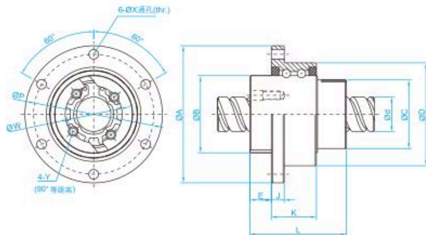
RSY Nut Rotating Ball Screw Specification and Dimension Table
