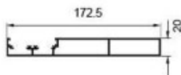
BF129 Triple side seal Weight: 1.533kg/m Thickness : 1.4mm
