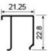
FG023B Clip Weight: 0.149kg/m Thickness : 0.8mm
