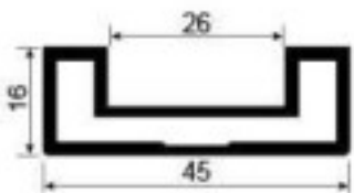
SK557 Vertical door frame Weight: 0.652kg/m Thickness : 2.0mm
