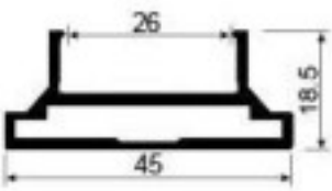
SK543H Vertical door frame Weight: 0.647kg/m Thickness : 2.0mm
