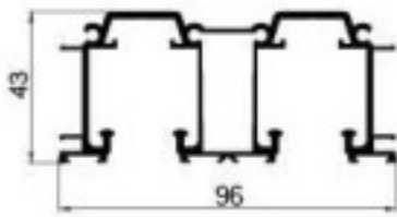
DX-89 Double hanging track Weight: 1.799kg/m Thickness : 1.8mm
