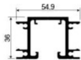
SG129 Single hanging track Weight: 1.197kg/m Thickness : 2.5mm
