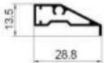
D-A619 F stripe Weight: 0.223kg/m Thickness : 1.0mm
