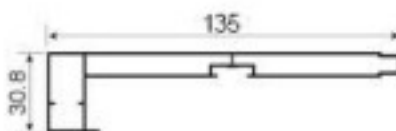
BT056 Door casing with trim Weight: 1.078kg/m Thickness: 1.1mm
