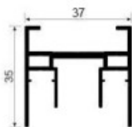
SK728 Top and bottom frame Weight: 0.691kg/m Thickness: 1.5mm
