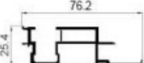
D-A633 Buffer upper horizontal frame Weight: 1.013kg/m Thickness : 1.6mm
