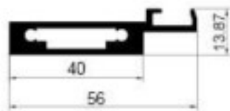
D-A622 Door frame Weight: 0.827kg/m Thickness : 2.0mm
