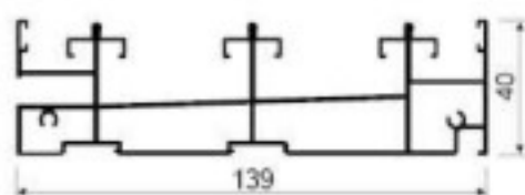
XG149 Triple high bottom track Weight: 2.173kg/m Thickness : 1.4mm
