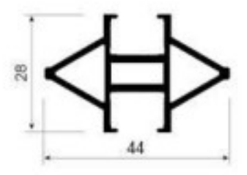
ZH186 Decorative strip Weight: 0.649kg/m Thickness : 2.0mm
