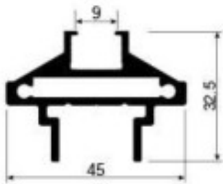
SK521 Top and bottom door frame Weight: 0.893kg/m Thickness : 2.0mm
