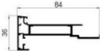
D-A625B Push in door jamb Weight: 1.135kg/m Thickness : 1.8mm
