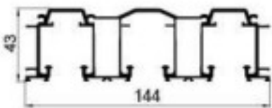
DX-90 Triple hanging track Weight: 2.525kg/m Thickness : 1.8mm
