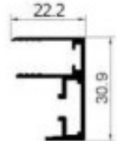
DX18A Trim Weight: 0.382kg/m Thickness : 1.5mm
