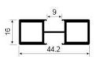
ZH190 Decorative strip Weight: 0.577kg/m Thickness : 1.4mm
