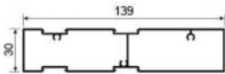
FG031 Triple center column Weight: 1.308kg/m Thickness : 1.2mm
