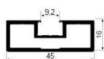
SK478H Vertical door frame Weight: 0.664kg/m Thickness : 2.0mm
