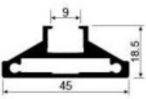
SK520 Vertical door frame Weight: 0.698kg/m Thickness : 2.0mm
