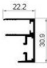
DX18A Trim Weight: 0.382kg/m Thickness : 1.5mm
