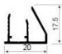
BT052 F strip Weight: 0.164kg/m Thickness : 1.0mm
