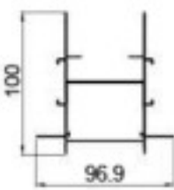
DX-60 Plaster single track profile Weight: 1.745kg/m Thickness : 2.0mm
