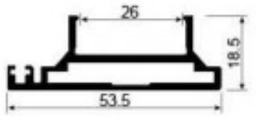
SK545H Door frame with hook Weight: 0.698kg/m Thickness : 2.0mm
