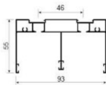
SG234 Double sliding track Weight: 1.265kg/m Thickness : 1.2mm
