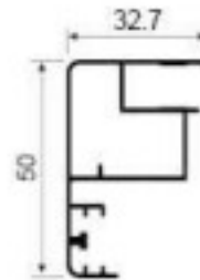
D-A531A Trim Weight: 0.521kg/m Thickness : 0.95mm
