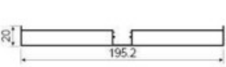
BF155 Four side seal Weight: 1.69kg/m Thickness : 1.4mm
