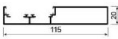
BF128 Double side seal Weight: 0.935kg/m Thickness : 1.2mm
