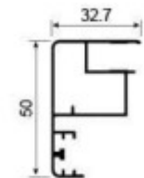
D-A531A Trim Weight: 0.521kg/m Thickness : 0.95mm
