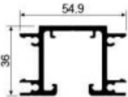
SG129 Top track Weight: 1.197kg/m Thickness : 2.5mm
