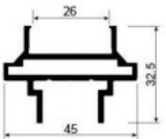
SK544H Top and bottom door frame Weight: 0.808kg/m Thickness : 2.0mm
