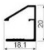
BT053 F strip Weight: 0.288kg/m Thickness : 1.0mm
