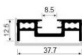
SK732A Vertical door frame Weight: 0.466kg/m Thickness: 1.5mm
