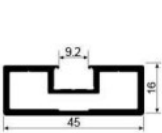
SK478H Vertical door frame Weight: 0.664kg/m Thickness : 2.0mm
