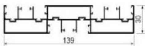
BF166 Triple side seal Weight: 1.954kg/m Thickness : 1.3mm
