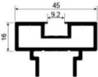
SK479H Top and bottom door frame Weight: 0.859kg/m Thickness : 2.0mm
