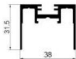
DX10 Bottom door frame Weight: 0.686kg/m Thickness : 1.9mm
