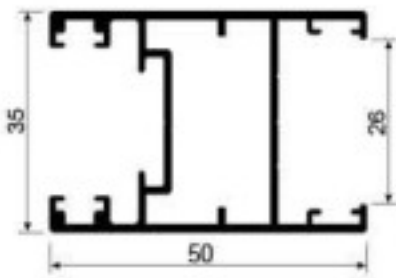
SK775 Vertical door frame Weight: 0.780kg/m Thickness : 1.4mm
