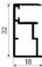
BT058H Trim Weight: 0.345kg/m Thickness : 1.2mm
