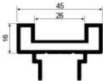
SK559 Top and bottom door frame Weight: 0.842kg/m Thickness : 2.0mm
