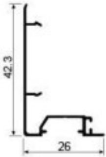
SK777 Door frame with hook Weight: 0.207kg/m Thickness : 0.8mm
