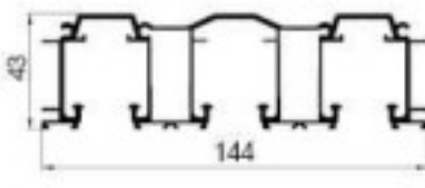
DX-90 Triple hanging track Weight: 2.525kg/m Thickness : 1.8mm
