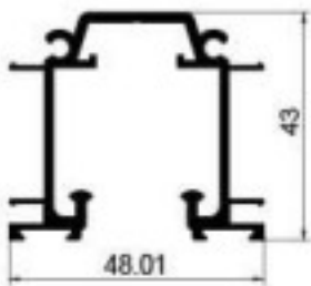
DX-88 Single hanging track Weight: 0.978kg/m Thickness : 1.8mm
