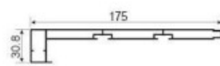
BT057 Door casing with trim Weight: 1.589kg/m Thickness: 1.3mm
