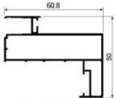
D-A615 Push in door jamb Weight:0.785kg/m Thickness :1.1mm
