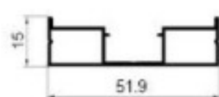
DX-94 Single side seal Weight: 0.430kg/m Thickness : 1.1mm
