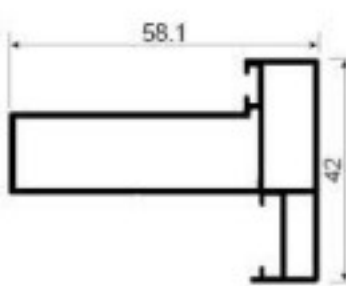
D-A613 Push in door jamb Weight: 0.756kg/m Thickness : 1.2mm
