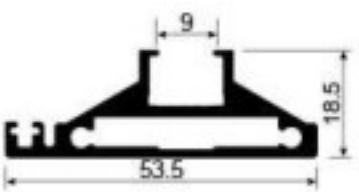
SK522 Door frame with hook Weight: 0.783kg/m Thickness : 2.0mm
