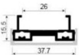
SK727 Vertical door frame Weight: 0.486kg/m Thickness: 1.5mm
