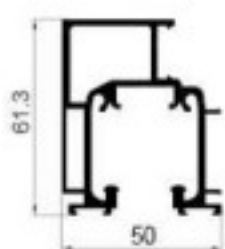
DX-52 Side hanging track Weight: 1.780kg/m Thickness : 2.5mm
