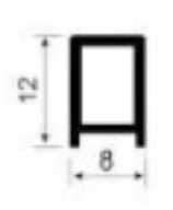
S472 Decorative strip Weight: 0.110kg/m Thickness : 1.2mm
