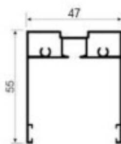
SG233 Single sliding track Weight: 0.782kg/m Thickness : 1.2mm
