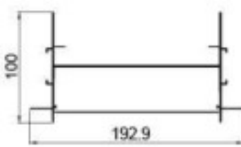
DX-62 Plaster triple track profile Weight: 2.673kg/m Thickness : 2.0mm
