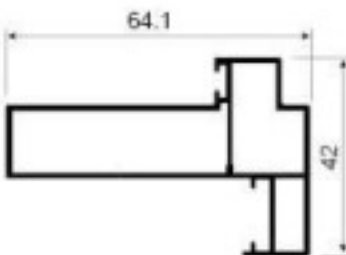
D-A563H Push in door jamb Weight: 0.800kg/m Thickness : 1.2mm
