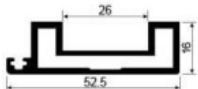
SK558 Door frame with hook Weight: 0.737kg/m Thickness : 2.0mm
