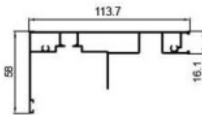
SG161 Four or 2+0 top track Weight: 1.431kg/m Thickness : 1.4mm
