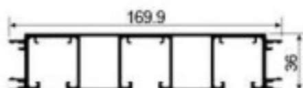
SG128 Triple hanging track Weight: 3.127kg/m Thickness : 2.5mm
