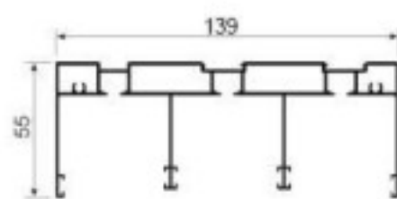
SG235 Triple sliding track Weight: 1.963kg/m Thickness : 1.3mm
