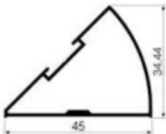
SK490 45 degrees corner Weight: 0.497kg/m Thickness : 1.0mm
