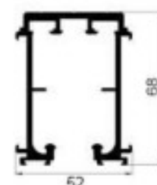
DX2 Pocket door track Weight: 1.966kg/m Thickness : 2.5mm
