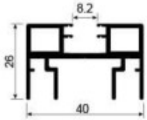
SK762H Top and bottom door frame Weight: 0.745kg/m Thickness : 1.5mm
