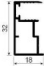
BT058H Trim Weight: 0.345kg/m Thickness : 1.2mm
