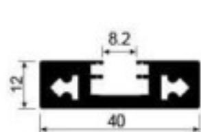
SK774 Vertical door frame Weight: 0.860kg/m Thickness : 3.5mm
