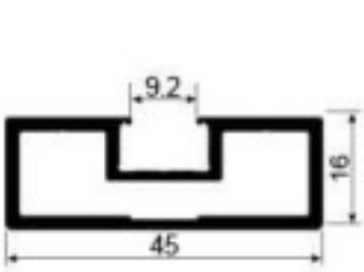
SK478H Vertical door frame Weight: 0.664kg/m Thickness : 2.0mm
