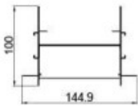
DX-61 Plaster double track profile Weight: 2.136kg/m Thickness : 2.0mm
