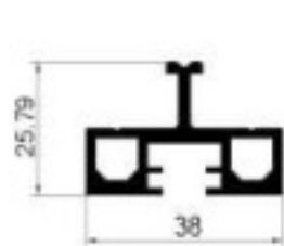
DX-83 Top door frame Weight: 0.788kg/m Thickness : 2.0mm
