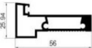
D-A624 Closing Weight: 0.883kg/m Thickness : 1.5mm
