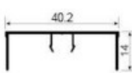
BF097A Triple side seal cover Weight: 0.204kg/m Thickness : 1.0mm
