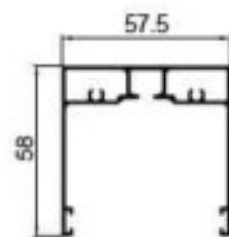
SG112 Single top track Weight: 0.907kg/m Thickness : 1.2mm
