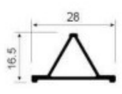
ZHT124 Decorative strip Weight: 0.196kg/m Thickness : 1.0mm
