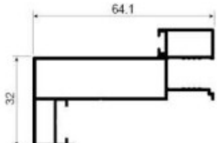
D-A562 Push in door jamb Weight: 0.841 kg/m Thickness: 1.2mm
