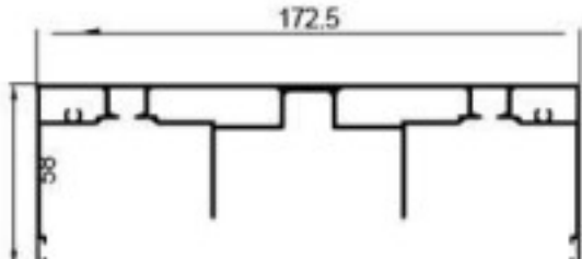
SG110 Triple top track Weight: 2.22kg/m Thickness : 1.4mm
