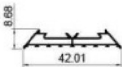
DX-87 Plaster middle cover Weight: 0.231kg/m Thickness : 0.7mm
