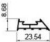
DX-86 Plaster side cover Weight: 0.139kg/m Thickness : 0.7mm
