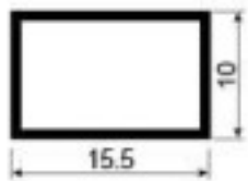
GB044 Double cover Weight: 0.104kg/m Thickness : 0.8mm
