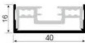
OPK-A203-40 Door frame Weight: 0.266kg/m Thickness: 1.5mm
