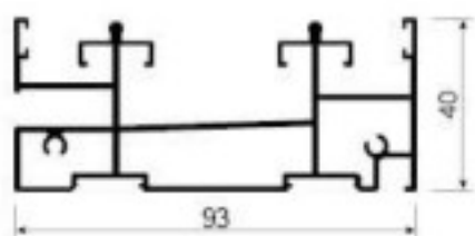
XG148 Double high bottom track Weight: 1.603kg/m Thickness : 1.4mm
