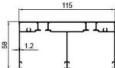
SG113 Double top track Weight: 1.588kg/m Thickness : 1.2mm
