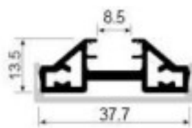
SK734A Vertical door frame Weight: 0.493kg/m Thickness: 1.5mm
