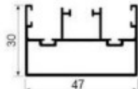
BF164 Single side seal Weight: 0.649kg/m Thickness : 1.2mm
