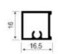
GT059 Lock material Weight: 0.21kg/m Thickness : 1.1mm
