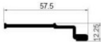
DX-72 Door trim profile Weight: 0.459kg/m Thickness : 2.3mm
