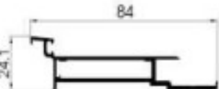
D-A626 Plaster frame Weight: 0.849kg/m Thickness : 1.8mm
