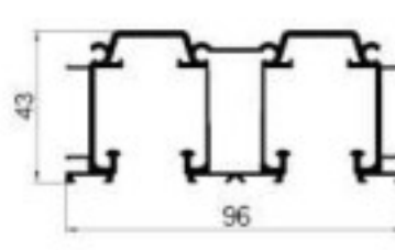
DX-89 Double hanging track Weight: 1.799kg/m Thickness : 1.8mm
