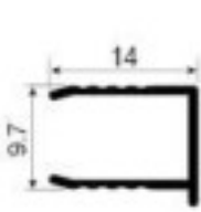
D-A550 F strip Weight: 0.088kg/m Thickness : 1.0mm
