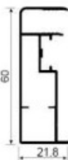
BT046 Trim Weight: 0.563kg/m Thickness : 1.1mm
