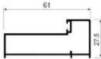
D-A566 Push in door jamb Weight: 0.609kg/m Thickness : 1.2mm
