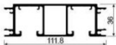
SG127 Double hanging track Weight: 1.83kg/m Thickness : 2.5mm
