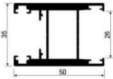
SK776 Vertical door frame Weight: 1.166kg/m Thickness : 4.0mm
