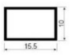
GT044 Window pane divider strip Weight: 0.104kg/m Thickness : 0.8mm
