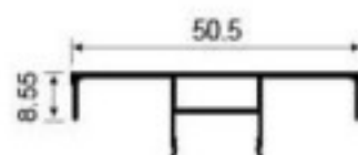
BF141 Side seal cover Weight: 0.292kg/m Thickness : 1.0mm
