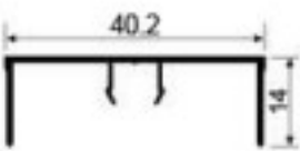
BF097A Triple side seal cover Weight: 0.204kg/m Thickness : 1.0mm
