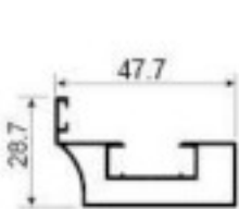
SK599 Closing Weight: 0.473kg/m Thickness : 1.0mm
