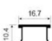
BF153 Side seal cover Weight: 0.090kg/m Thickness : 1.2mm
