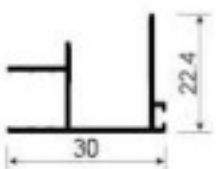
OPK-A329 Frames Weight: 0.232kg/m Thickness: 1.0mm
