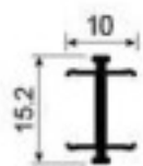
SG160B Connecting strip Weight: 0.099kg/m Thickness : 1.6mm
