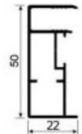
H682A Trim Weight: 0.500kg/m Thickness : 1.1mm
