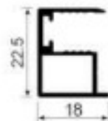
D-A548H Trim Weight: 0.268kg/m Thickness : 1.2mm
