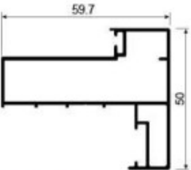
D-A614 Push in door jamb Weight: 0.769kg/m Thickness : 1.1mm
