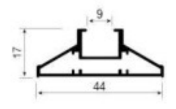
ZHT125 Decorative strip Weight: 0.385kg/m Thickness : 1.0mm
