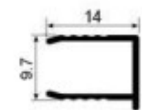
D-A550 F strip Weight: 0.207kg/m Thickness : 0.8mm
