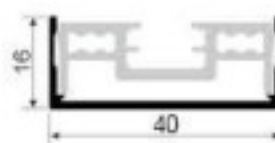
OPK-A203-40 Door frame Weight: 0.266kg/m Thickness: 1.5mm
