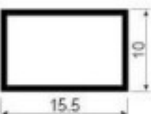
GB044 Window pane divider strip Weight: 0.104kg/m Thickness : 0.8mm
