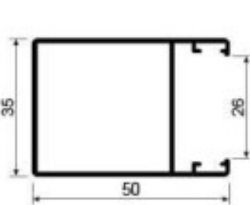
SK780 Door frame Weight: 0.599kg/m Thickness : 1.2mm
