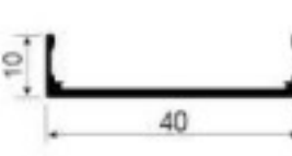
OPK-A229 Door frame Weight: 0.219kg/m Thickness: 1.5mm
