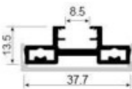
SK733A Vertical door frame Weight: 0.470kg/m Thickness: 1.5mm
