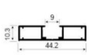
ZHT126H Decorative strip Weight: 0.336kg/m Thickness : 1.0mm
