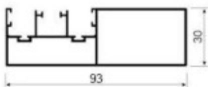
BF165 Double side seal Weight: 1.047kg/m Thickness : 1.2mm
