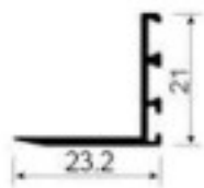
OPK-A308A Cancealed track cover Weight: 0.174kg/m Thickness : 1.0mm
