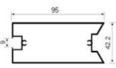
ZHT128 Lock profile Weight: 1.260kg/m Thickness : 1.5mm
