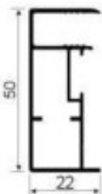
H682A Trim Weight: 0.500kg/m Thickness : 1.1mm
