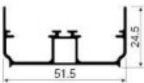
SK485A Lock profile for 1+1 Weight: 0.497kg/m Thickness : 1.0mm
