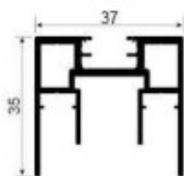
SK731A Top and bottom frame Weight: 0.772kg/m Thickness: 1.5mm
