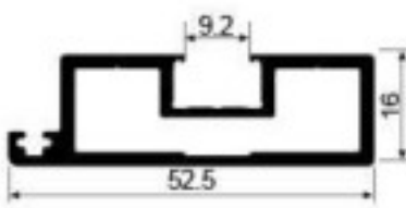
SK480H Door frame with hook Weight: 0.733kg/m Thickness : 2.0mm
