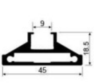
SK520 Vertical door frame Weight: 0.698kg/m Thickness : 2.0mm
