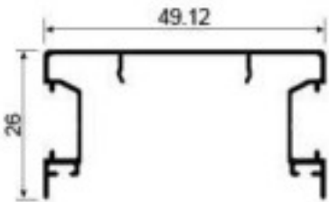
SK778 Door frame with hook Weight: 0.316kg/m Thickness : 0.8mm
