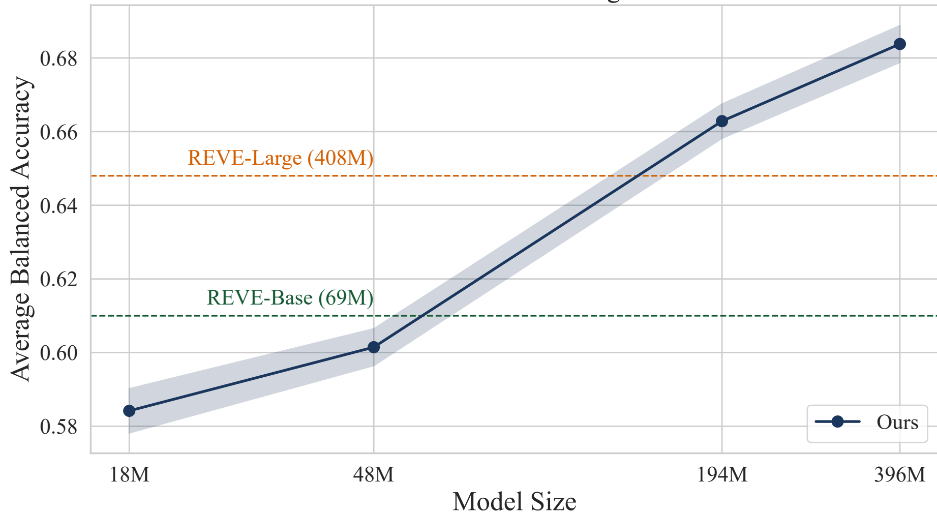
Model Size Scaling
