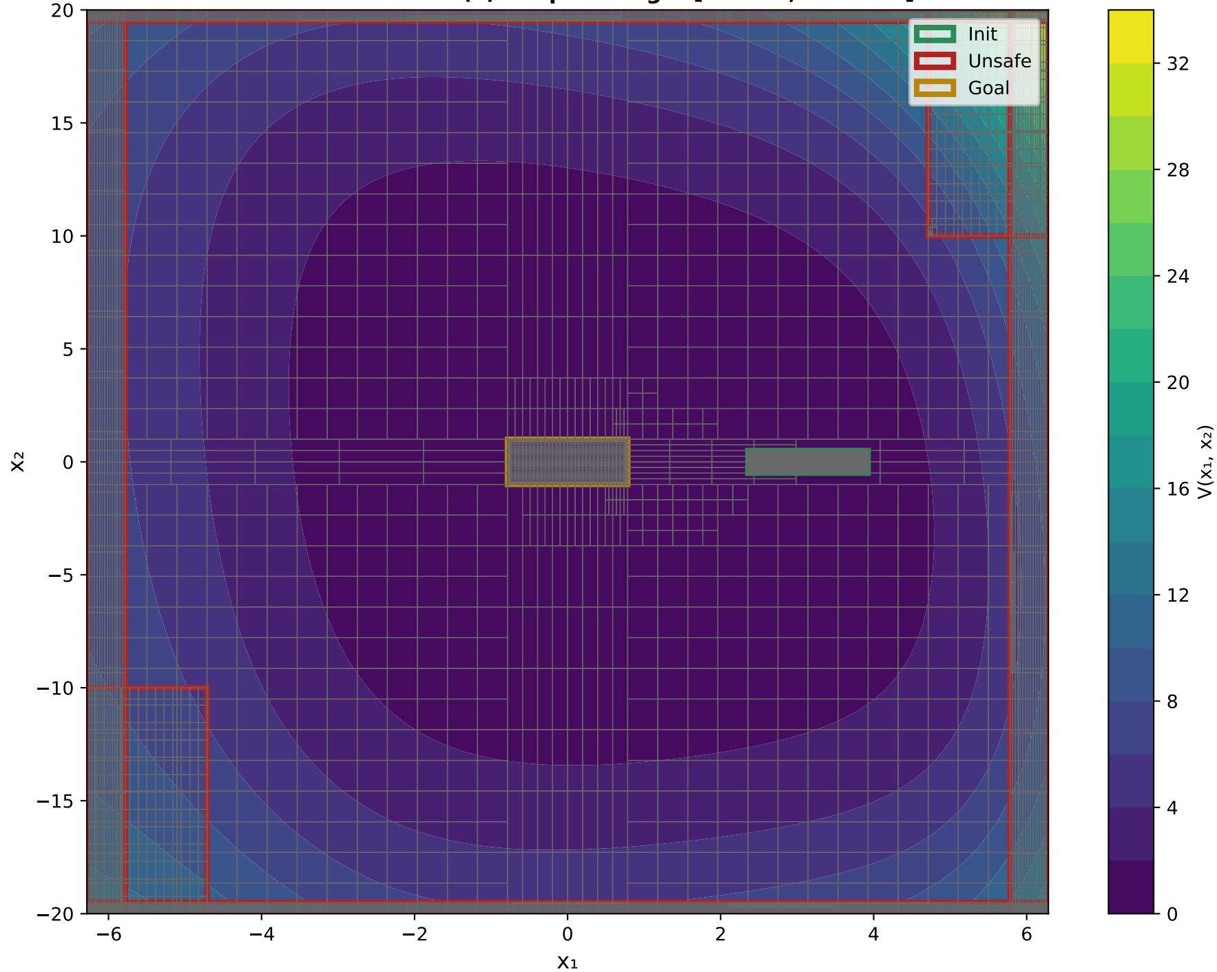
X 1 VS X 2 Final Evaluation - V(x) Output Range: [0.0959, 32.7781]
