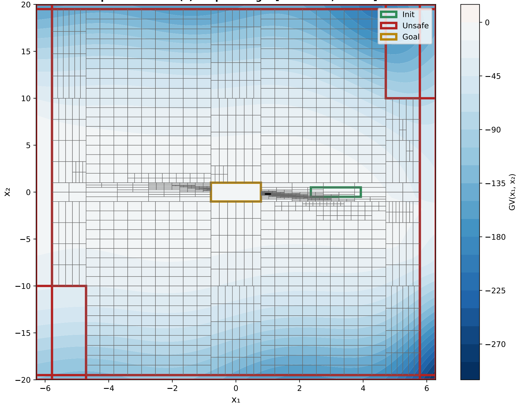
X 1 VS X 2 Epoch 2000 - GV(x) Output Range: [-289.1853, 0.0022]
