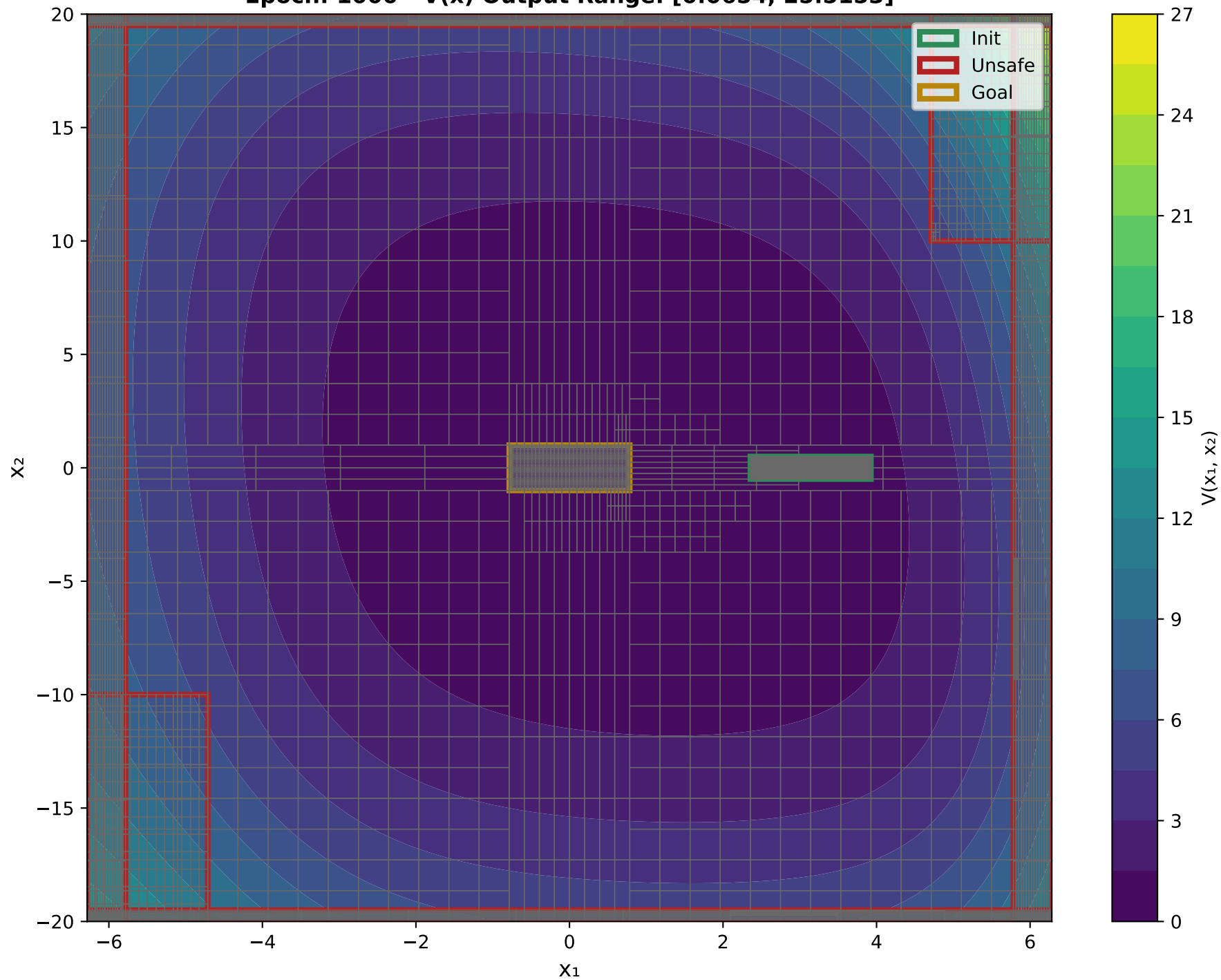
X 1 VS X 2 Epoch: 1000 - V(x) Output Range: [0.0654, 25.5153]
