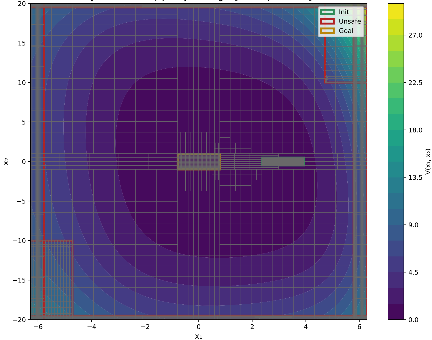
X 1 VS X 2 Epoch: 2000 - V(x) Output Range: [0.0701, 29.5728]
