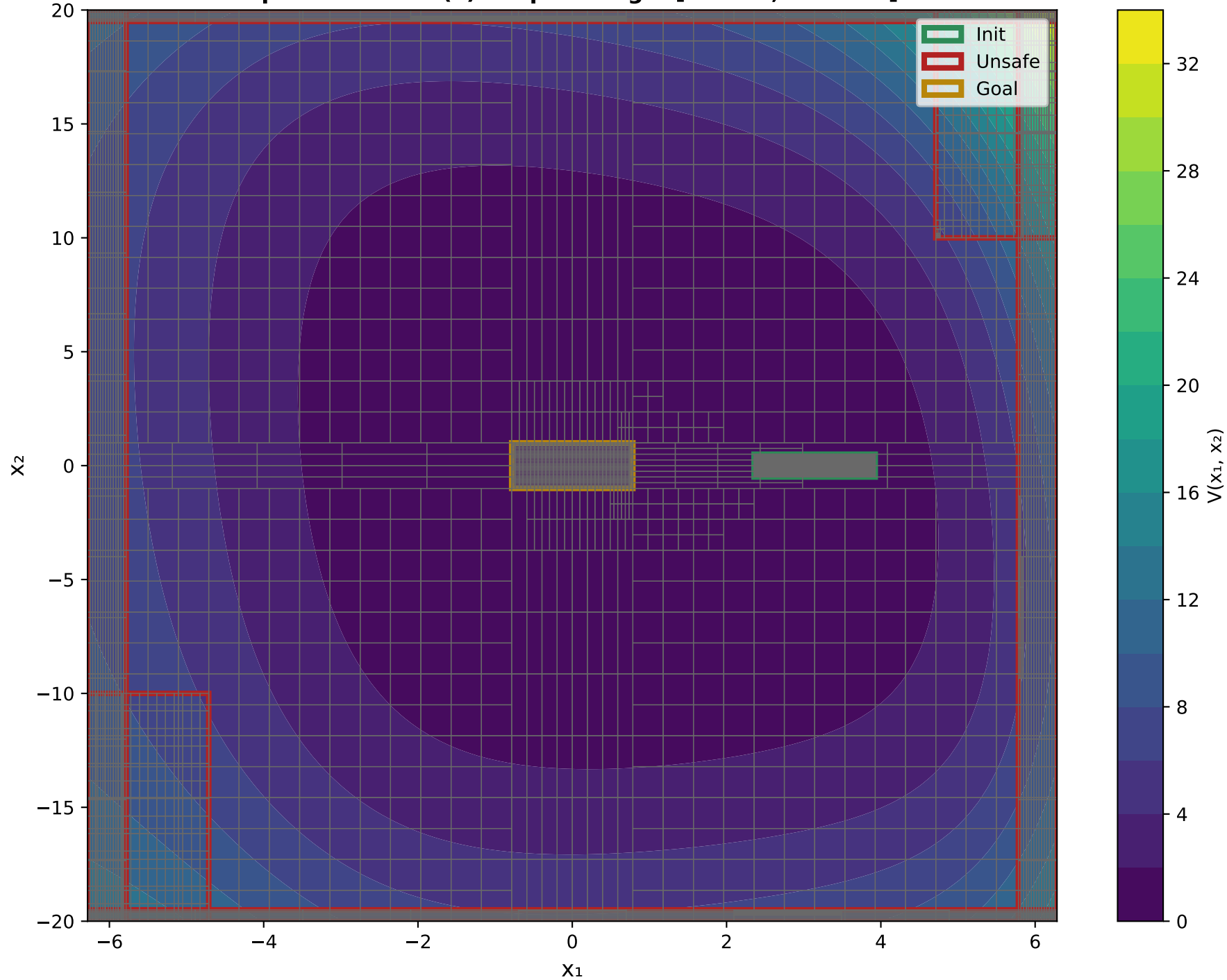
X 1 VS X 2 Epoch: 3000 - V(x) Output Range: [0.0924, 32.5397]
