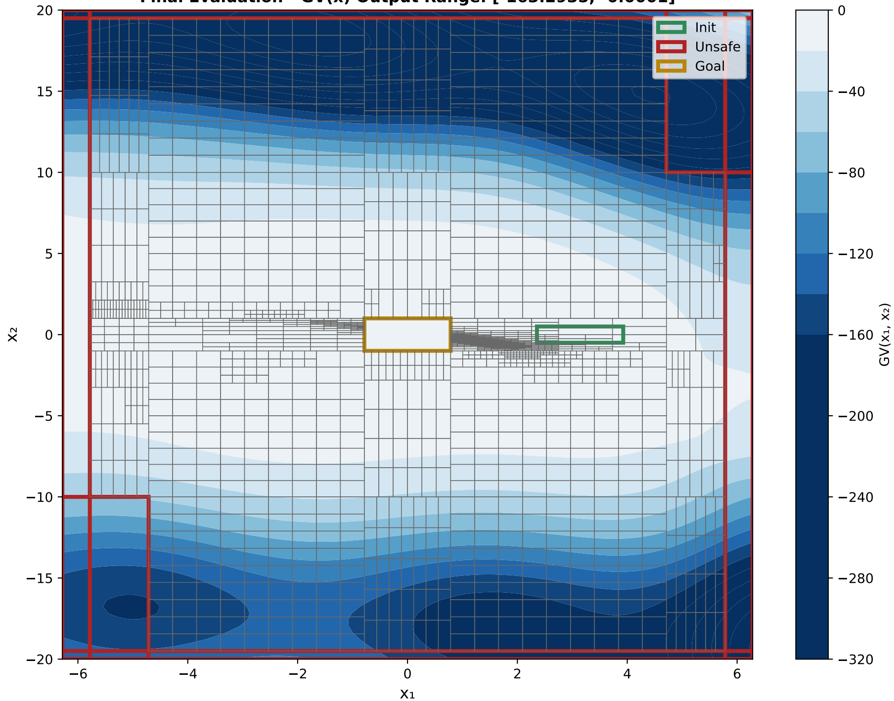
X 1 VS X 2 Final Evaluation - GV(x) Output Range: [-163.2935, -0.0001]
