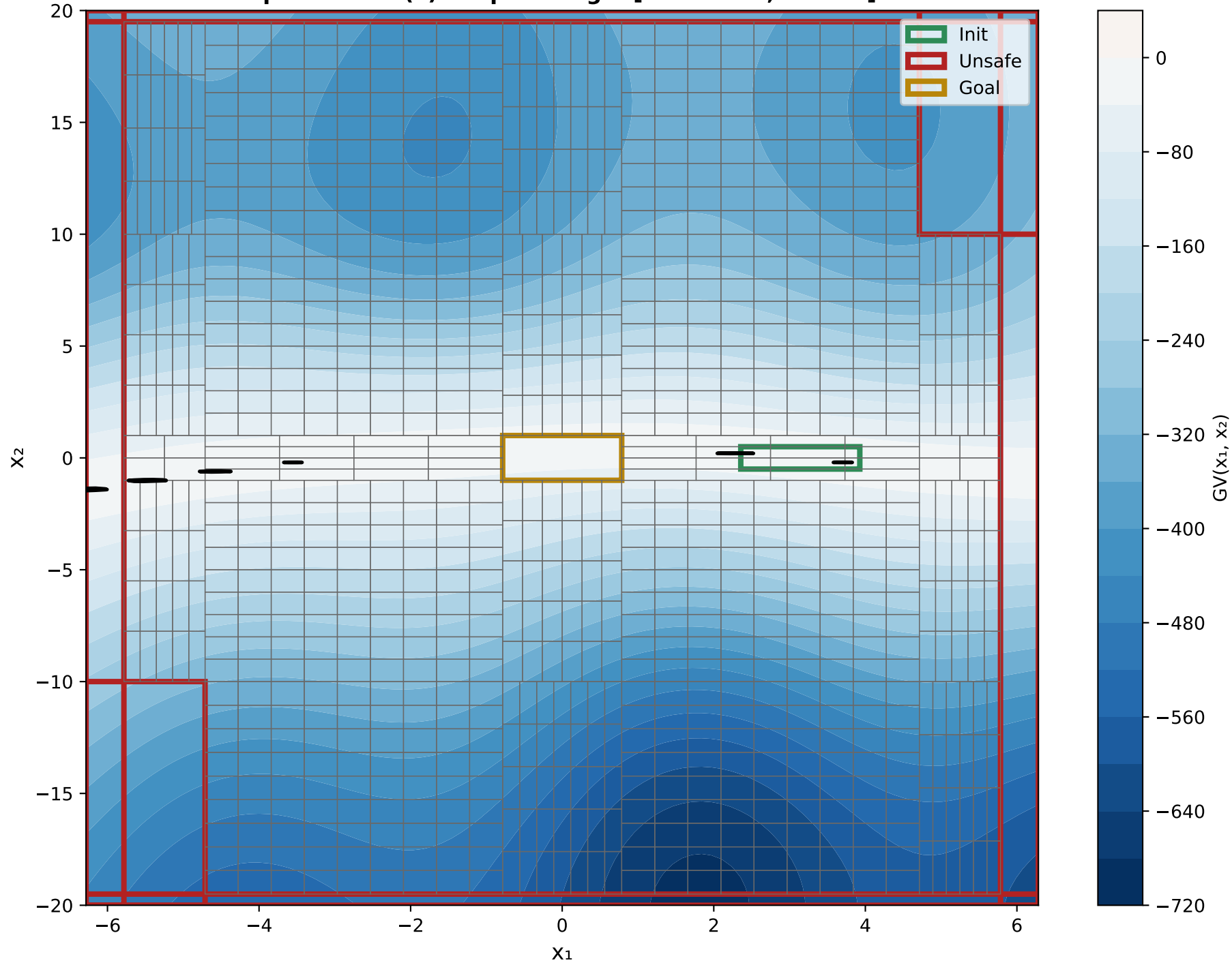
X 1 VS X 2 Epoch 0 - GV(x) Output Range: [-694.2963, 1.0165]
