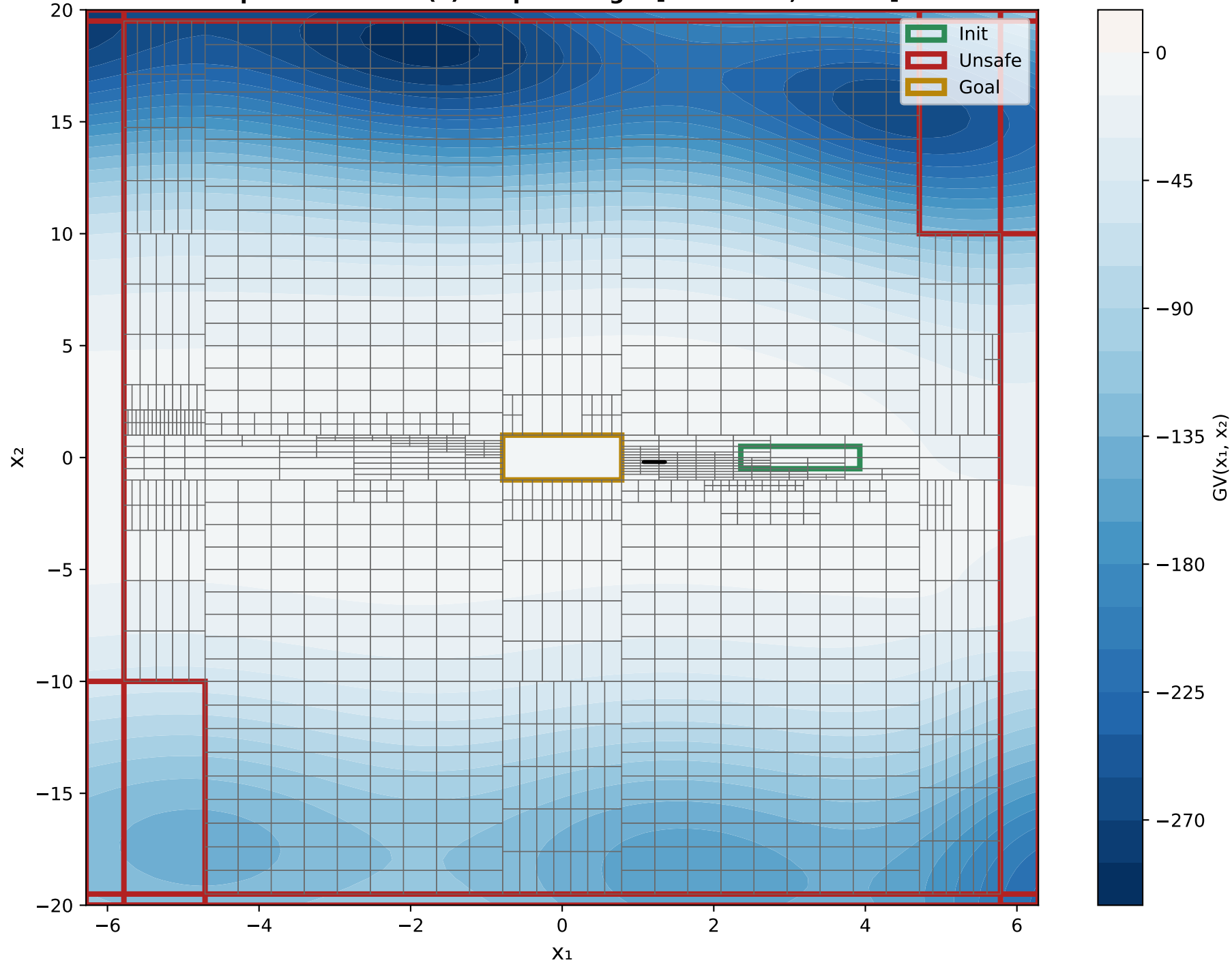
X 1 VS X 2 Epoch 1000 - GV(x) Output Range: [-292.1789, 0.0049]
