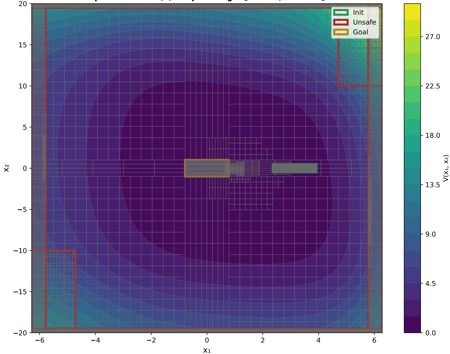
X 1 VS X 2 Epoch: 3000 - V(x) Output Range: [0.0643, 28.9441]
