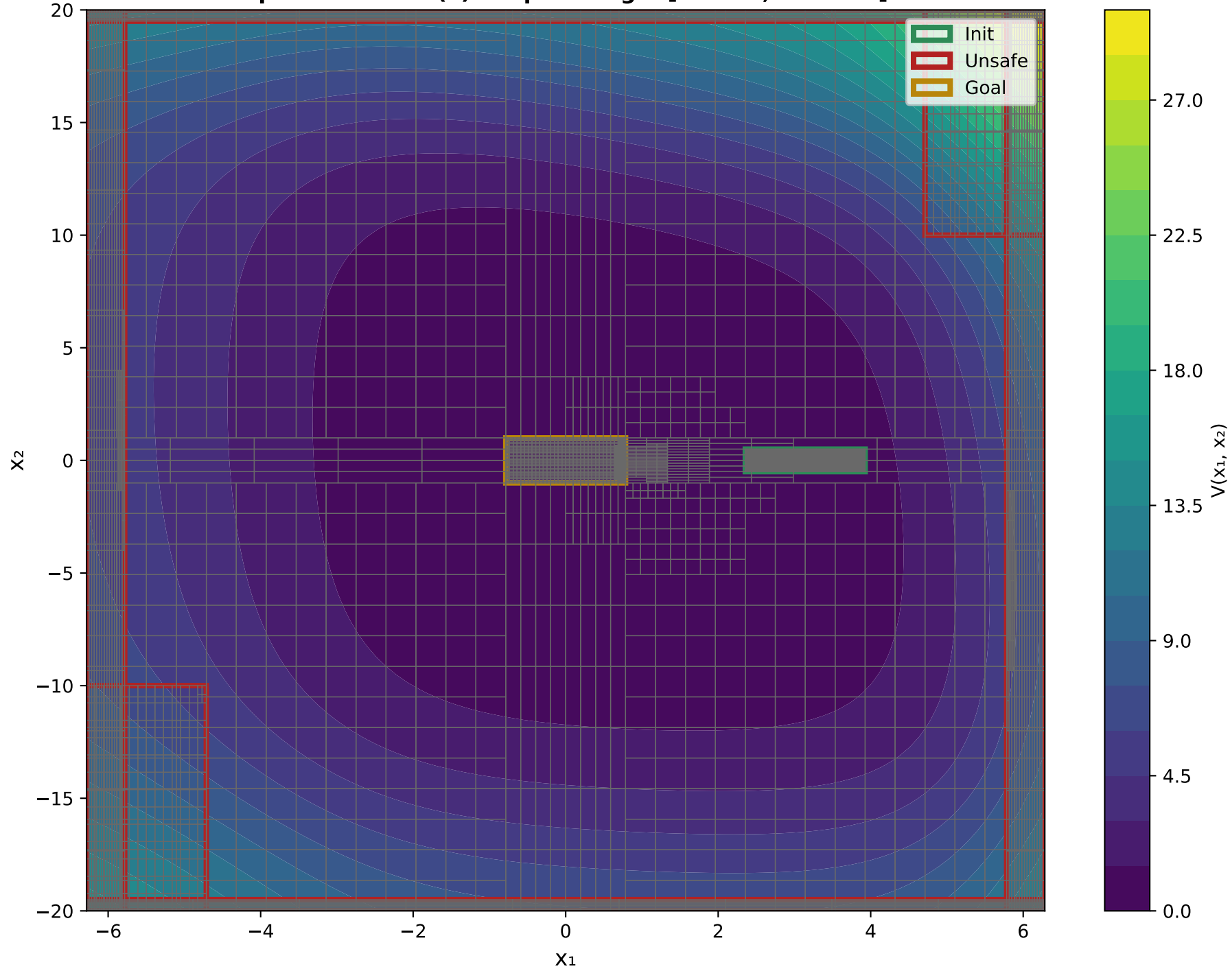
X 1 VS X 2 Epoch: 4000 - V(x) Output Range: [0.0887, 29.8094]
