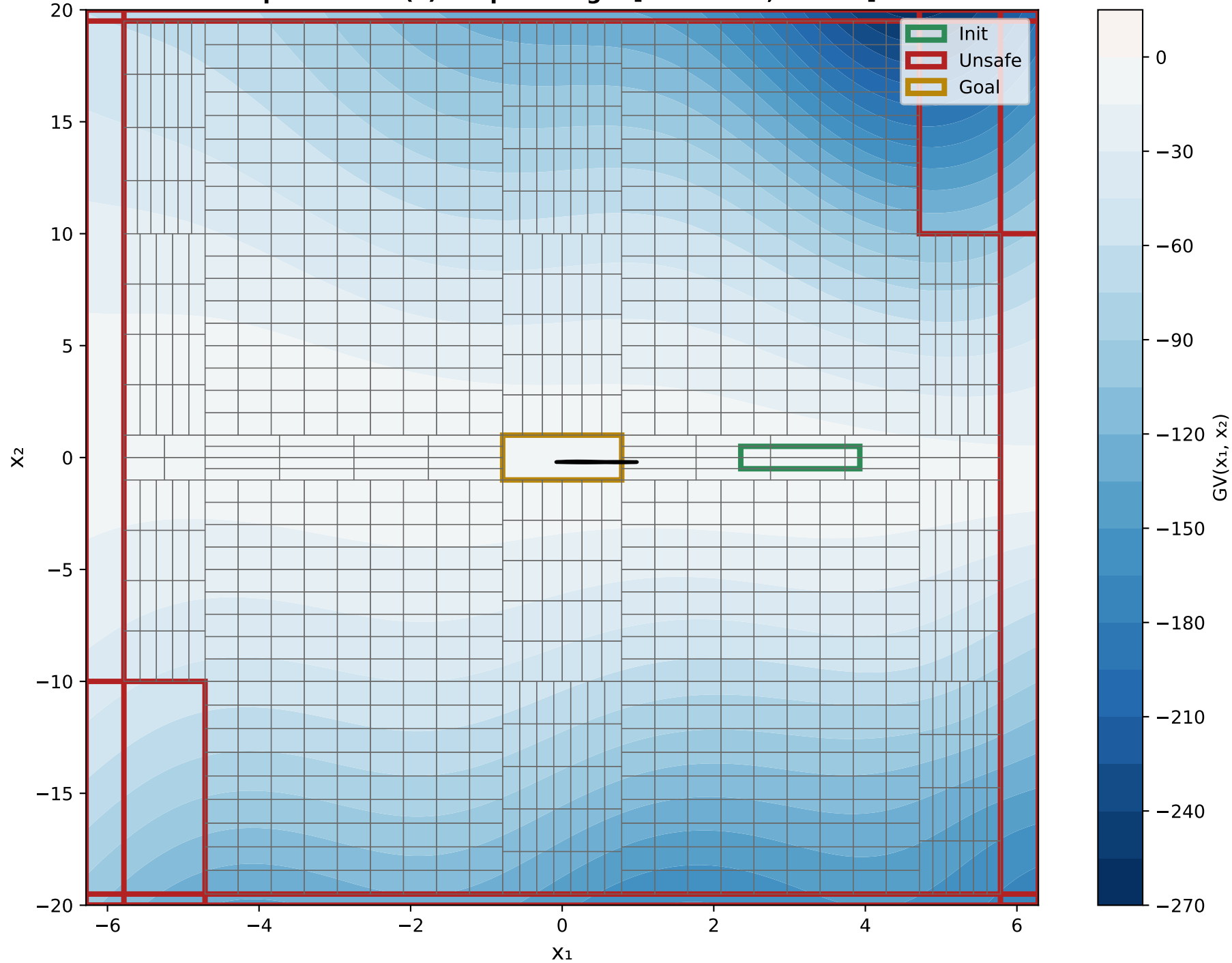
X 1 VS X 2 Epoch 0 - GV(x) Output Range: [-260.3110, 0.0501]
