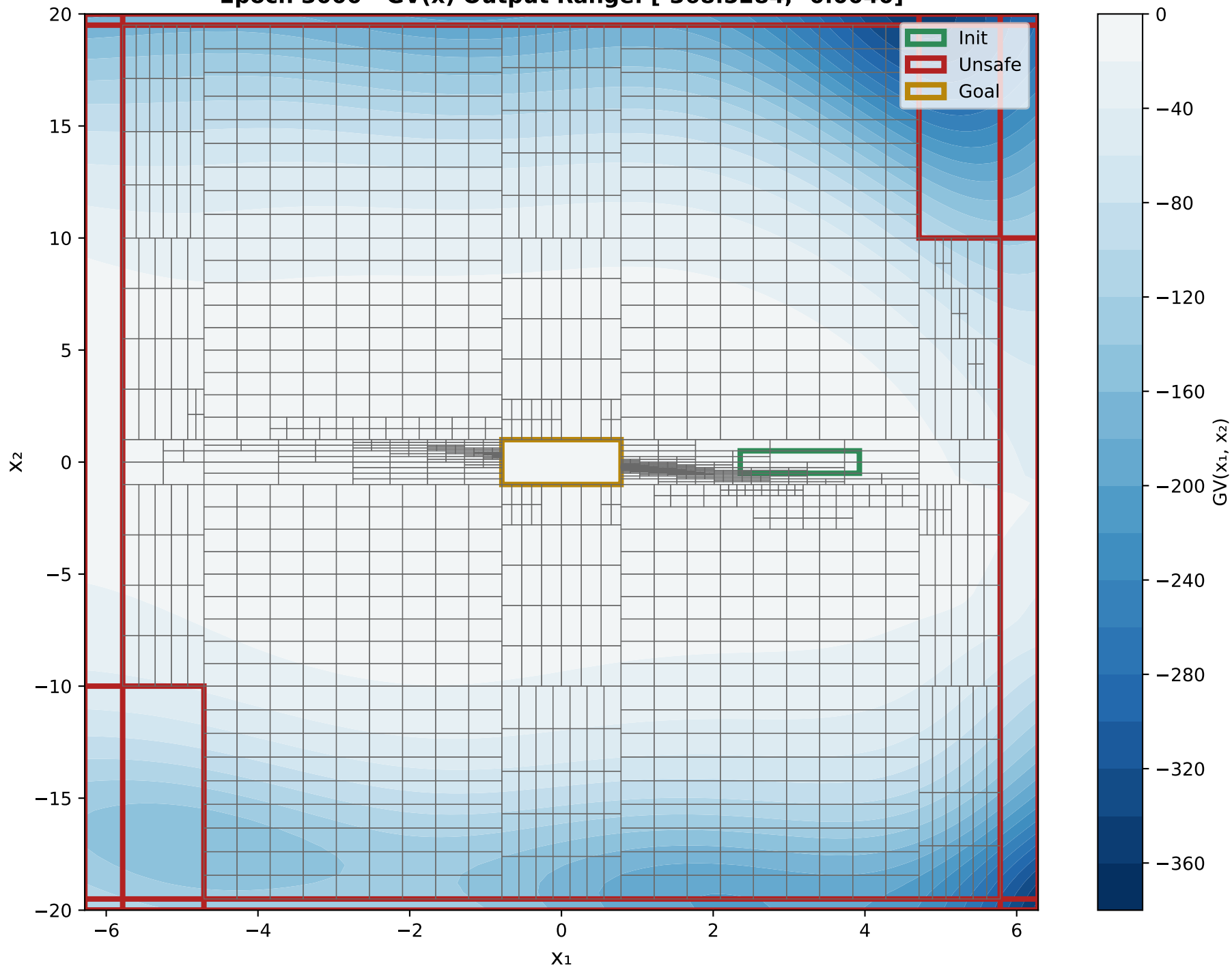
X 1 VS X 2 Epoch 3000 - GV(x) Output Range: [-368.5284, -0.0040]
