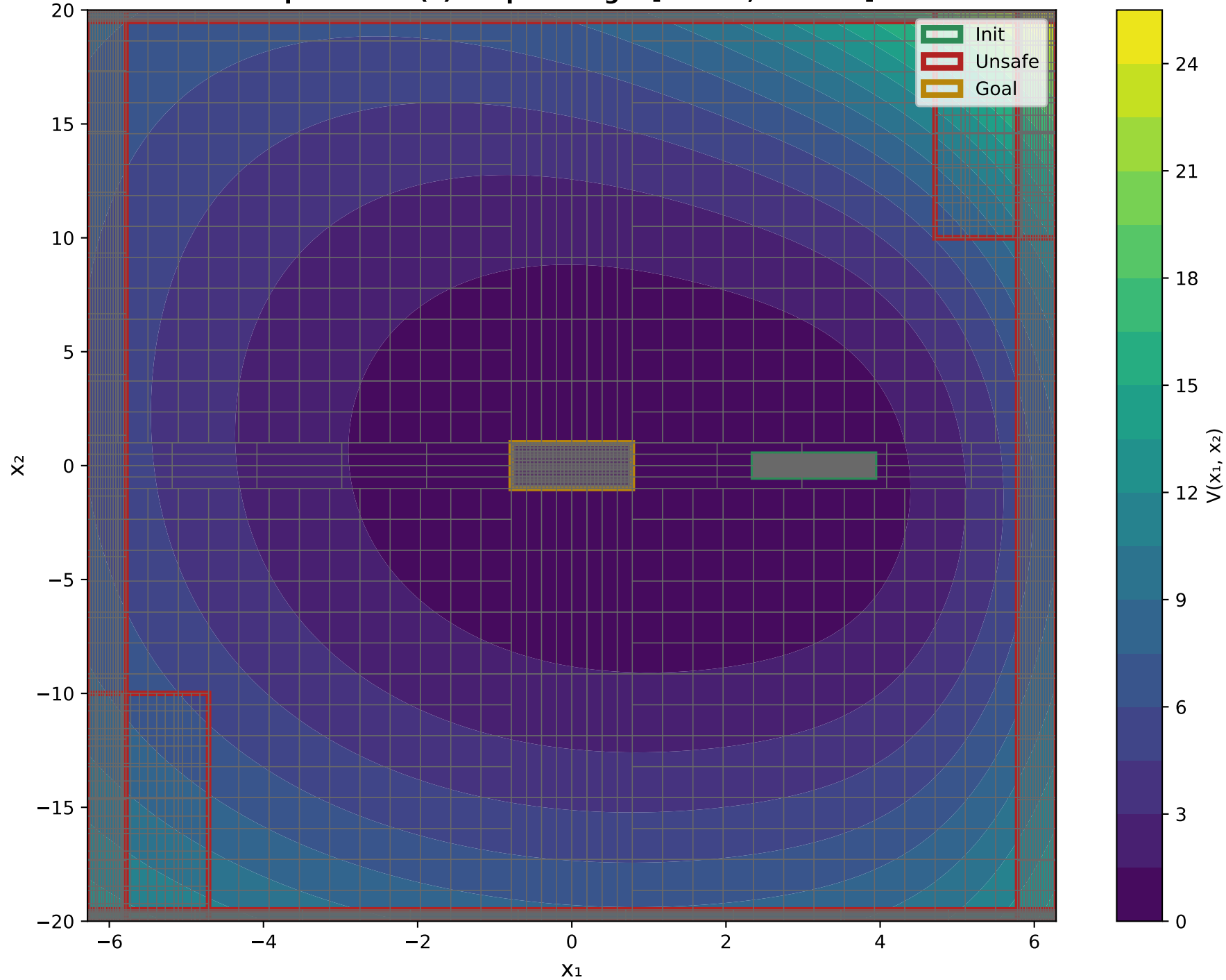
X 1 VS X 2 Epoch: 0 - V(x) Output Range: [0.0064, 25.4982]
